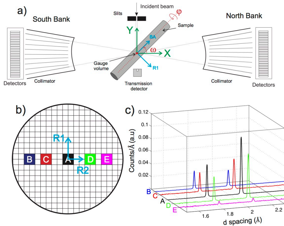
Figure 1 (a) Schematic diagram of the ENGIN-X time-of-flight neutron strain scanner, with a bolt at the sample position. (b) Explored locations on the HMS Pomone bolt cross section (grid spacing 1mm) (c) Diffactograms collected in the bolt axis direction from different locations across the bolt diameter.
