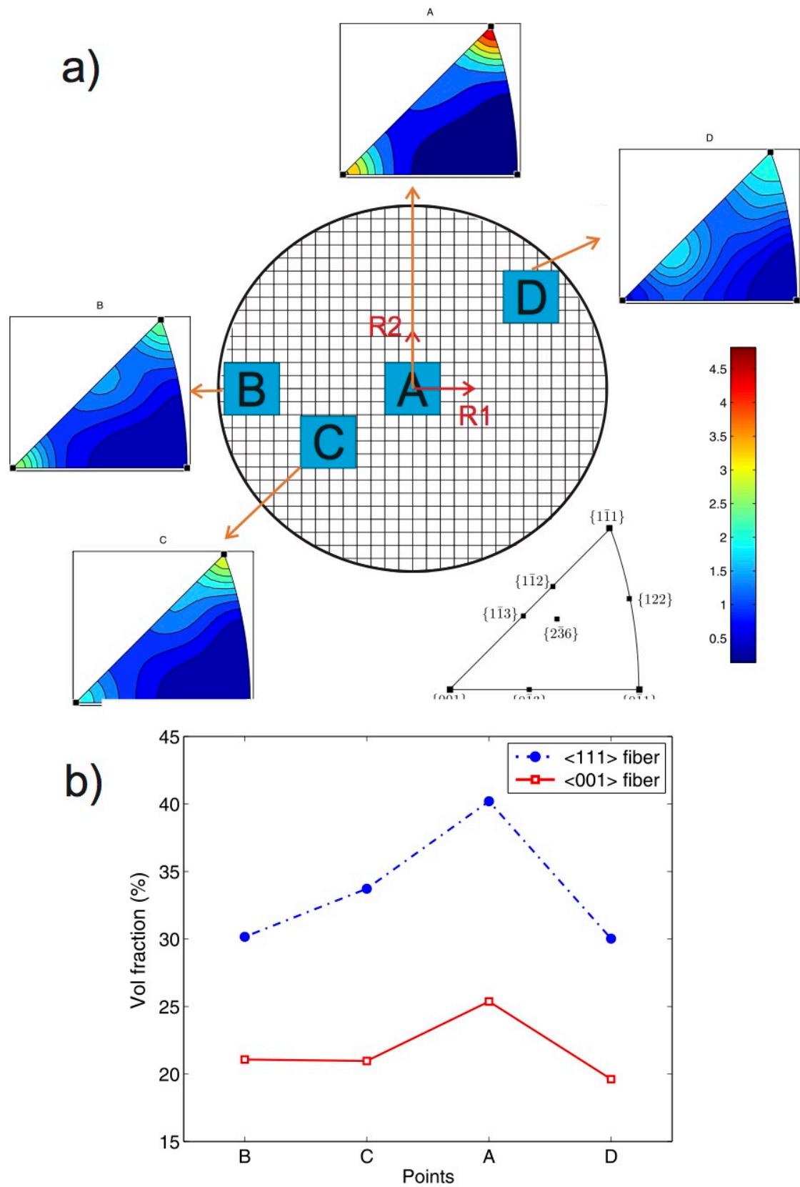
Figure 7 a) Inverse pole figures from each measurement volume in the HMS Amethyst bolt (grid spacing 1mm). All use the same colour scale in mrd. b) <111> and <001> fibre component volume fractions for different locations across the HMS Amethyst bolt diameter.
