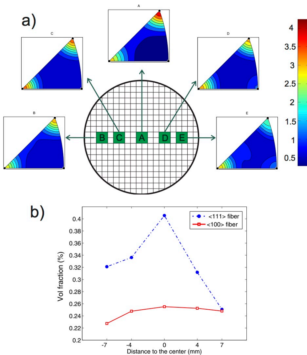
Figure 9 a) The recalculated inverse pole figures along the bolt axis direction (BA) for each point across the Pomone bolt segment diameter (grid spacing 1mm). b) <111> and <100> fibre component volume fractions for different locations across the segment sample diameter.
