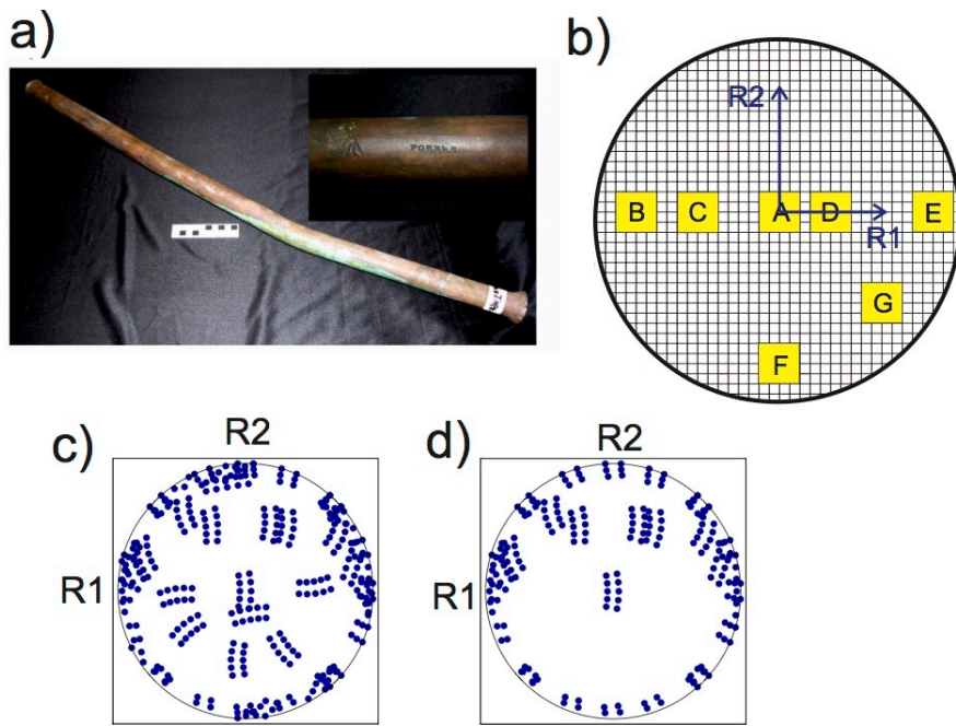
Figure 3 a) HMS Impregnable bolt with a Forbes works stamp b) Explored positions across the bolt cross section (grid spacing 1mm). c) Stereogram showing the expected pole figure coverage achieved by the chosen texture strategy for point A d) Expected pole figure coverage for other positions across the bolt cross section.
