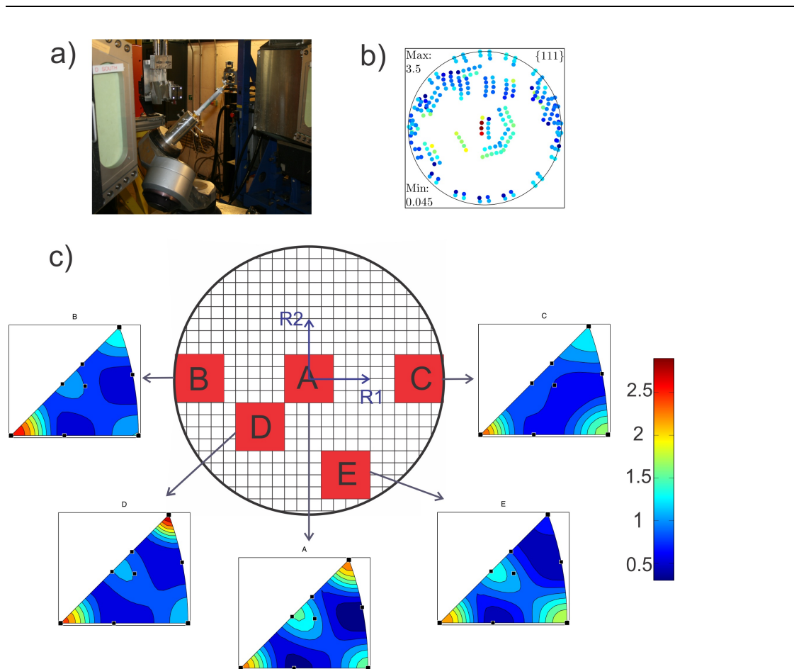
Figure 10 a) Photo of the Pomone bolt AB1-02-01 in ENGIN-X b) Position A {111} experimental pole figure. c) Inverse pole figures from each measurement volume in the Pomone bolt (grid spacing 1mm). All use the same colour scale in multiples of a random distribution
