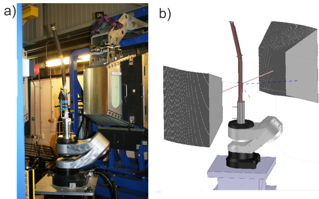
Figure 2 a) Experimental setup for the HMS Impregnable copper bolt using the Cybaman goniometer for \chi = 0^\circ, \omega = 0^\circ, \varphi = 0^\circ b) Screen capture of the corresponding SScanSS simulation, including calibrated sample positioning system, laser scanned sample model and ENGIN-X detector banks.
