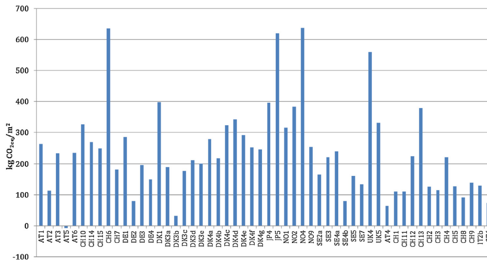
Fig. 5. Cradle-to-gate (A1-A3) EG from available Annex 57 case studies in kg CO 2eq /m 2 . [29].
