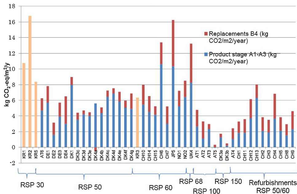
Fig. 6. Cradle-to-gate (A1-A3) + replacement (B4) EG from available Annex 57 case studies. Orange bars indicate case studies where reported results are a sum of production and replacement impacts. (For interpretation of the references to colour in this figure legend, the reader is referred to the web version of this article.)
