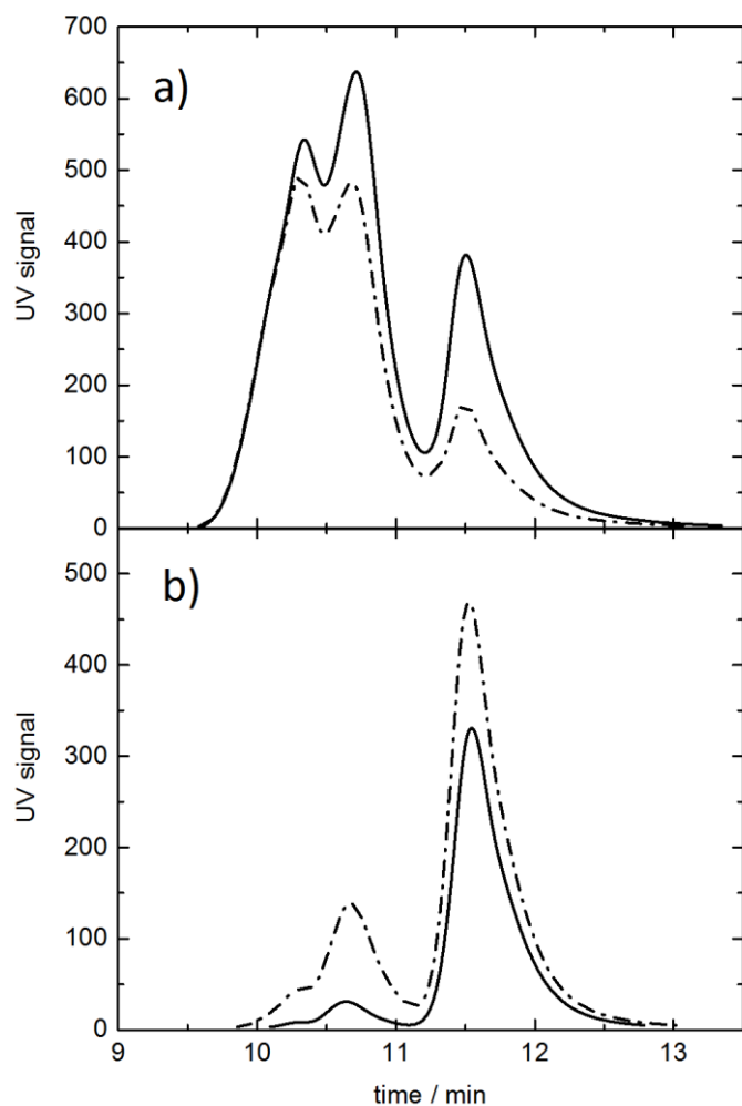
Figure 6. Comparative GPC analysis of the products from the extraction of bio-oil aq-E using: (—): scCO 2 , (---): Toluene. a) residue, b) extract.
