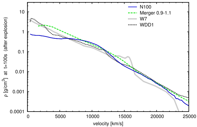
Figure 2. The N100 density profile (Seitzzahl et al. 2013) used as input data for our radiative-transfer calculations (dark blue, solid line). For comparison, we show the density of a white dwarf merger [ 0.9 M_{\odot} and 1.1 M_{\odot} C/O white dwarfs, Pakmor et al. (2012) and Röpke et al. (2012) – light green, dash-dotted line]. We furthermore show models of Nomoto et al. (1984) and Iwamoto et al. (1999), W7 (1D fast deflagration – grey, broad/micro-dashed line) and WDD1 (1D delayed detonation – black, dashed line), which have been used in many previous spectral modelling studies.
