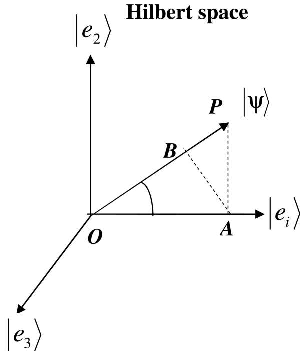
Fig. 1 Hilbert space analysis in which perpendiculars (like AB) are drawn from tips of components along eigen vectors to the normalized general state of the system |\psi\rangle to know the contributions (like OB) along the direction of |\psi\rangle
