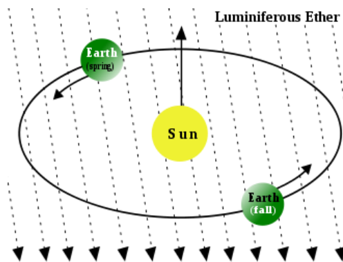
Figure 2. Luminiferous ether 4
