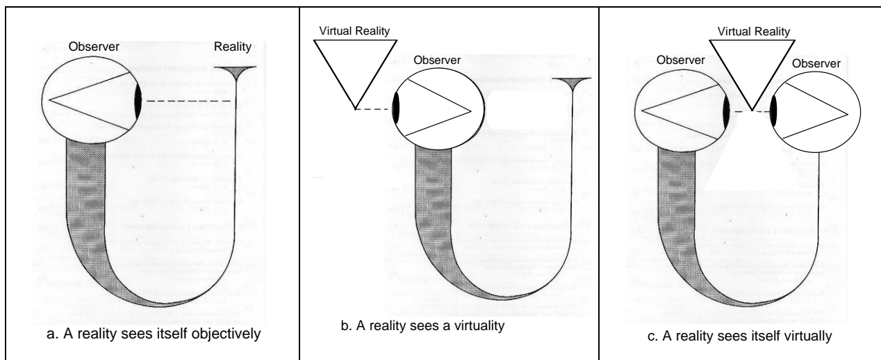
Figure 4. Reality models
