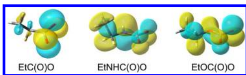
Figure 1. DFT-computed SOMOs of \text{Z-CO}_2^\bullet radicals.
