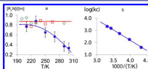
Figure 3. (a) Temperature dependence of [\mathbf{6}]/[\mathbf{Im}] ratios: blue ●, \text{PeBnN}^\bullet ( 6g ); red □, \text{Bn}_2\text{N}^\bullet ( 6d ); green ◇, (\text{allyl})_2\text{N}^\bullet ( 6f ). (b) Arrhenius plot of k_c for 6g .
