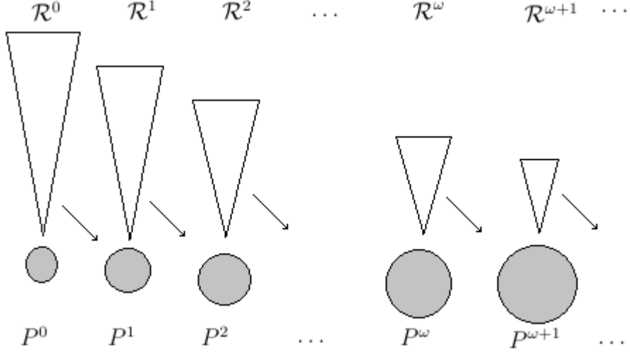
Figure 2: The Yablo sequence
