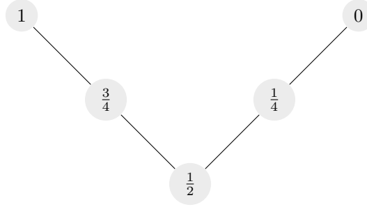
Figure 1: The ordering of the semantic values
