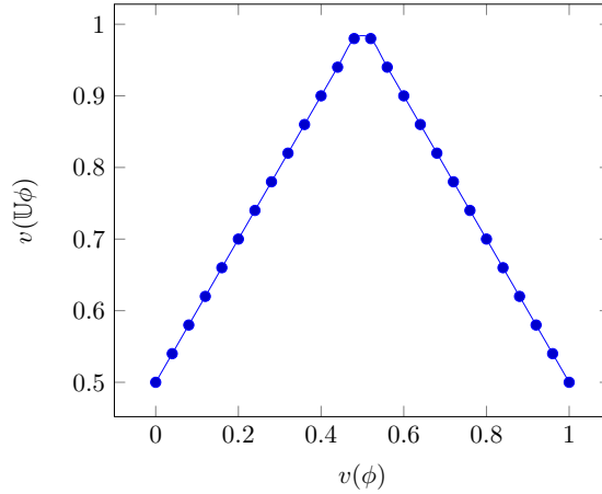
Figure 3: The unclarity operator \mathbb{U}
