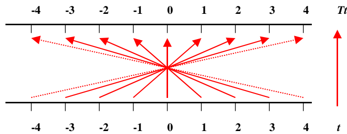
Point-to-point reflection mapping of moments. T: t \rightarrow -t .
