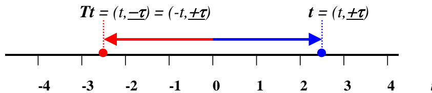
Vector reflection mapping. T: (t, \underline{+t}) \rightarrow (t, \underline{-t})
