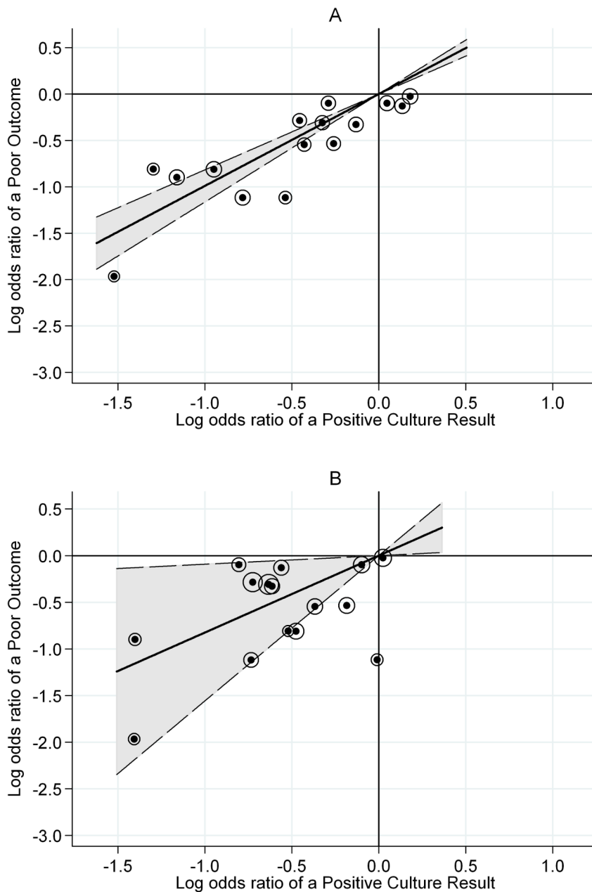
Figure 3. Sub-group analysis by geographical region: Hong Kong trials. A. Month 2 restricted to Hong Kong trials, R^2_{\text{trial}}=0.86 . B. Month 3 restricted to Hong Kong trials, R^2_{\text{trial}}=0.62 . Logs odds ratio of a poor outcome plotted against log odds ratio of a positive culture. Fitted line is weighted by the precision of the estimates, and this precision is represented by the diameter of the circles around each point. The dotted line represents the 95% confidence interval on the slope. doi:10.1371/journal.pone.0063840.g003
