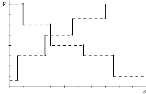
(a) \underline{a} = \bar{a} = \underline{b} < \bar{b}
