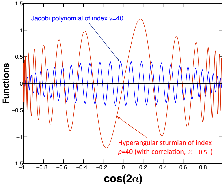
Figure 2. (Color on line) Plot of the Jacobi polynomial of index 40 (blue line) and the hyperangular sturmian function of index 40 and \mathcal{Z} = 0.5 for l_1 = l_2 = 0 as a function of \cos(2\alpha) . 503 B-splines have been used to generate the hyperangular sturmian function.
