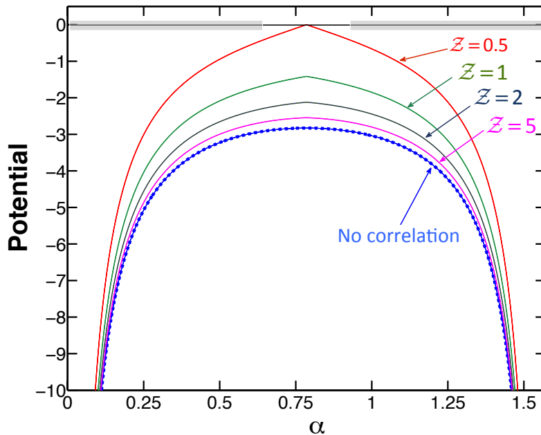
Figure 1. (Color on line) Plot of the potential term in the Schrödinger equation (27). This potential term is actually the effective charge \tilde{C}(\alpha) represented here for various values of \mathcal{Z} . The dashed (blue) line is obtained by neglecting v_0(\alpha) , the radial electronic repulsion. The nodes of the hyperangular sturmians concentrate in the shaded area on the horizontal axis.
