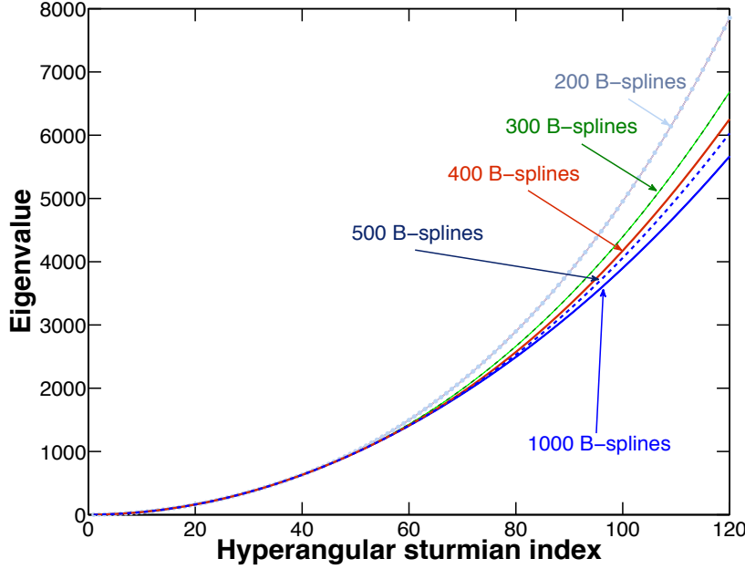
Figure 4. (Color on line) Eigenvalue of the corresponding hyperangular sturmian H_p^{0,0}(\alpha) eigenfunction solution of the Sturm-Liouville problem (22). The various curves correspond to different sizes of the B-spline basis in term of which these hyperangular sturmian functions are expanded.
