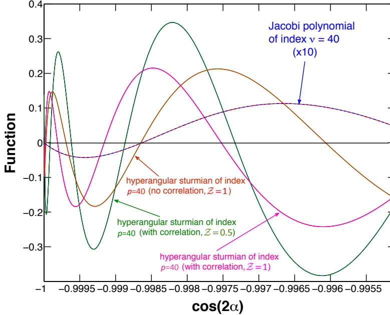
Figure 3. (Color on line) Plot of the Jacobi polynomial (multiplied by 10) of the same index 40 and l_1 = l_2 = 0 as a function of \cos 2\alpha very close to \cos(2\alpha) = -1 (blue dashed line). This Jacobi polynomial is compared to three hyperangular sturmian functions of index 40 and l_1 = l_2 = 0 : the red line corresponds to \mathcal{Z} = 1 within the independent model; the green line corresponds to \mathcal{Z} = 0.5 with correlation; the magenta line corresponds to \mathcal{Z} = 1 with correlation. As in Table II, 503 B-splines have been used to generate the hyperangular sturmians.
