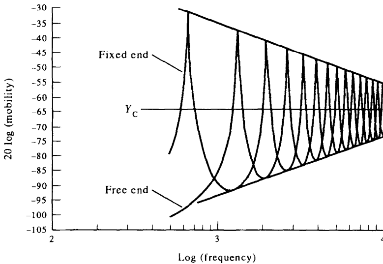
Fig. 2. Point mobility of end-excited rods with clamped and free ends.
