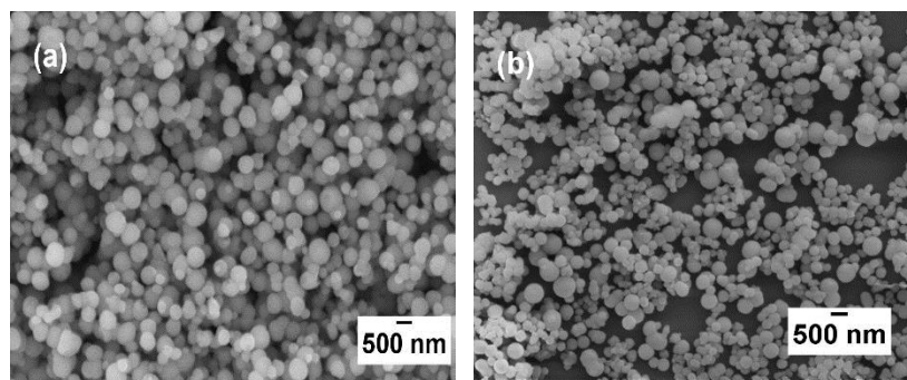
Figure 2. SEM images for the synthesised (a) pristine MCM-48 and (b) QAS-modified MCM-48.
