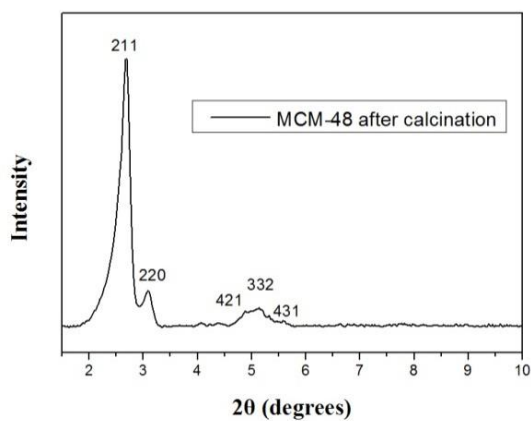
Figure 1. XRD patterns for the synthesised MCM-48 mesoporous nanoparticles, planes (211), (220), (421), (332) and (431) correspond to the cubic space group Ia3d.
