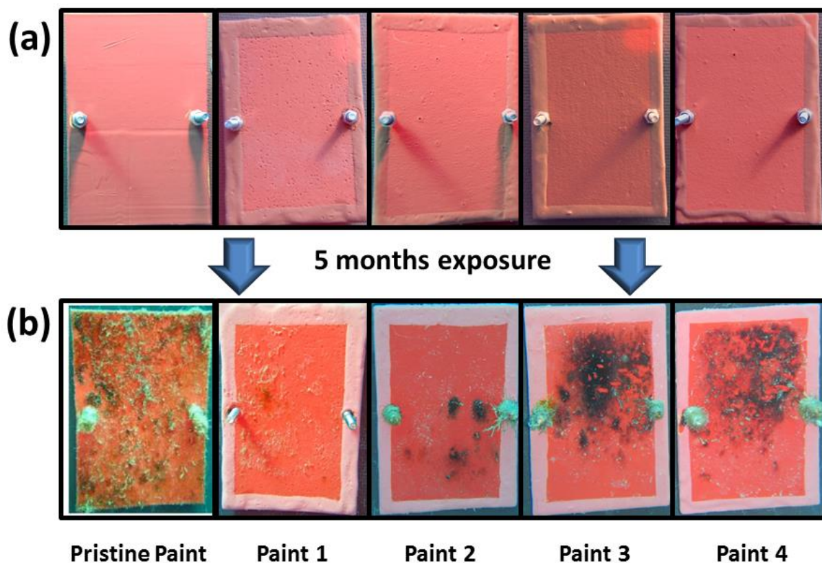
Figure 8. Photographs of PVC panels coated with Pristine Paint and Paints 1-4 for the field test trial (Eilat, northern Red Sea) in the first day of deployment (a) and after 5 months of exposure (b).
