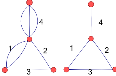
Figure 1: Multigraph and its underlying graph
