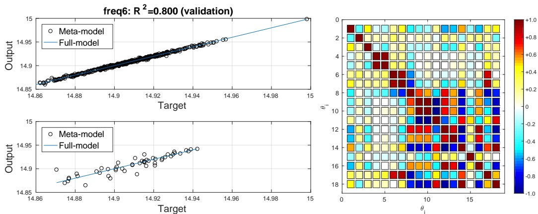
Fig. 3. Worst performance of the ANN configuration #9 (left panel) and predicted correlation among the outputs (right panel).
