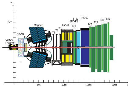
Figure 1: The LHCb detector - starting at the interaction point and proceeding downstream, we have the Vertex Locator, RICH1, TT, Magnet, T1-T2-T3 tracking stations, RICH2, Calorimeters and finally Muon chambers.
