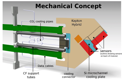
Figure 4: A conceptual 3D model of the mechanical design of a VELO upgrade module (subject to change).
