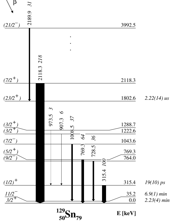
FIG. 1. Partial level scheme of ^{129}\text{Sn} [8] populated from the mixture of the three \beta -decaying isomers of ^{129}\text{In} indicating the \gamma -rays relevant to the analysis. The intensities obtained in the present experiment are given relative to the 315-keV \gamma ray.
