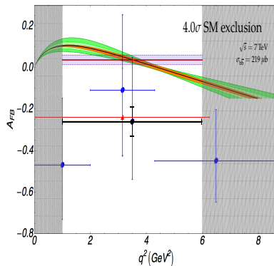
Figure 5: The precision on \mathcal{A}_{FB} expected from the LHCb experiment with 1\text{fb}^{-1} integrated luminosity. The present central value given by the Belle experiment is shown with a purely statistical uncertainty. The shaded bands show the theory expectation in the SM with uncertainties (orange), additional \Lambda/m_B corrections at the 10% level (green) and the average over the 1 < q^2 < 6 \text{ GeV}^2 region (pink). Taken from Ref. [20].
