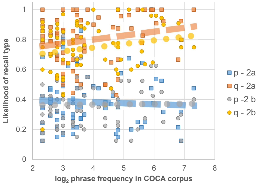
Figure 5: Comparison of Experiments 2a and 2b. The effect of phrase frequency is similar in both Experiment 2a and 2b for both the likelihood of remembering either one or two words (p) and for the likelihood of remembering two words when at least one word was recalled (q). Participants are less likely to recall phrases completely in Experiment 2b, the experiment in which they were prompted to only write down words rather than phrases.
