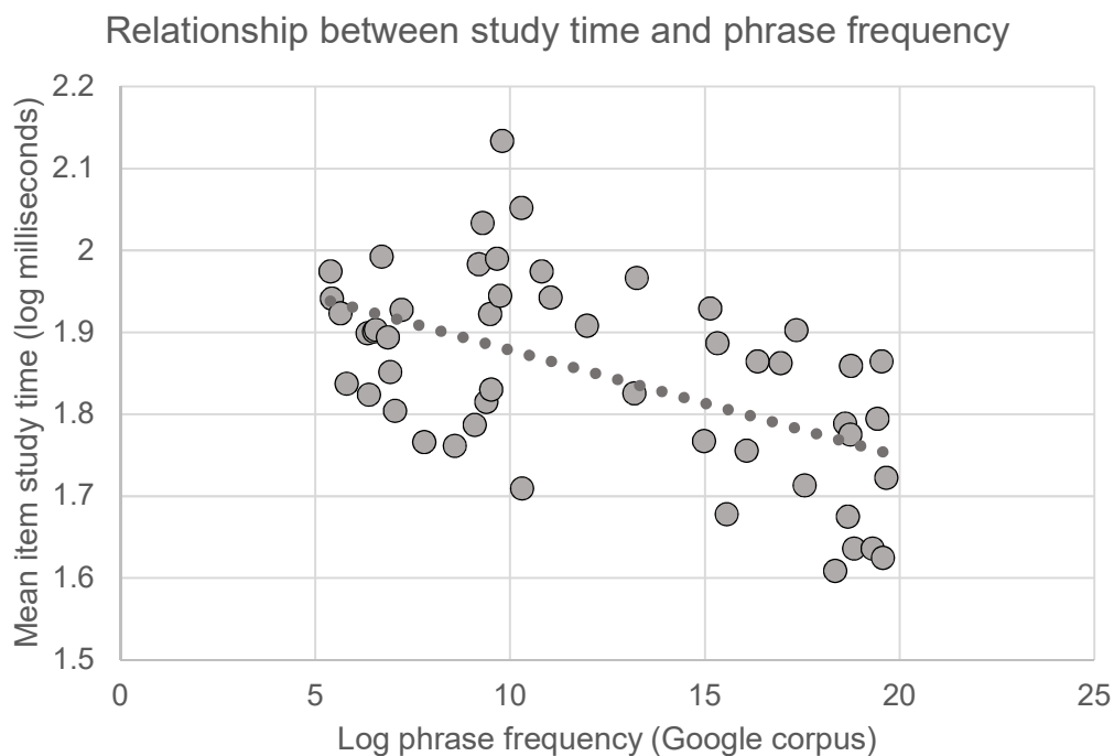
Figure 6: Effect of phrase frequency on study time. More common phrases are studied for less time.
