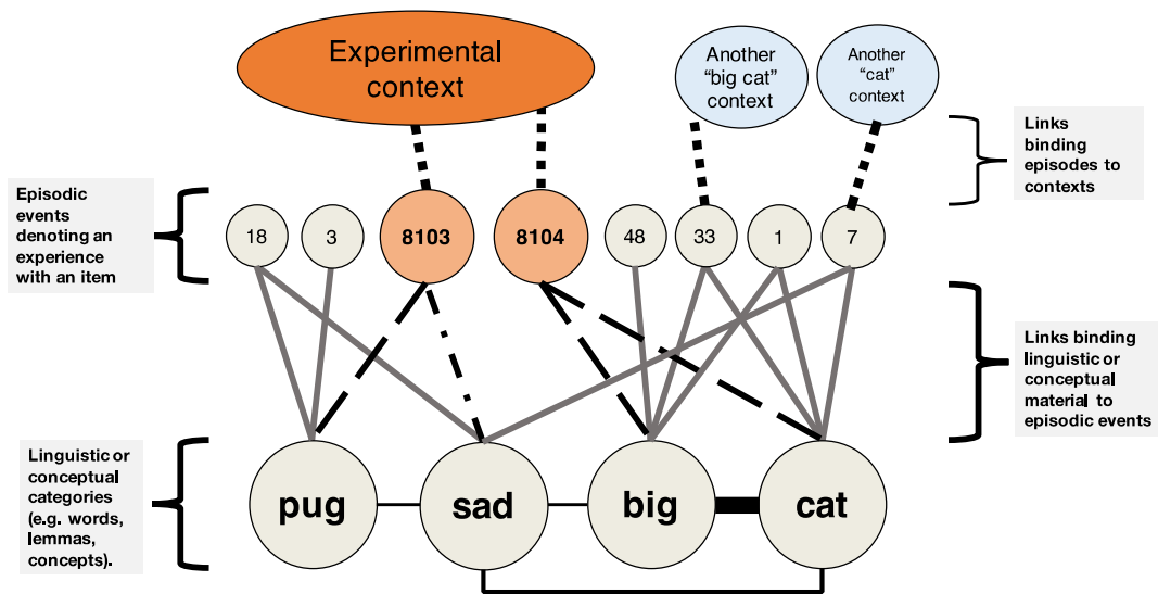
Figure 8: Diagram of the model of phrase frequency effects in recall and recognition. Frequent phrases are associated with more episodes and with stronger associations within the lexical-semantic network.
