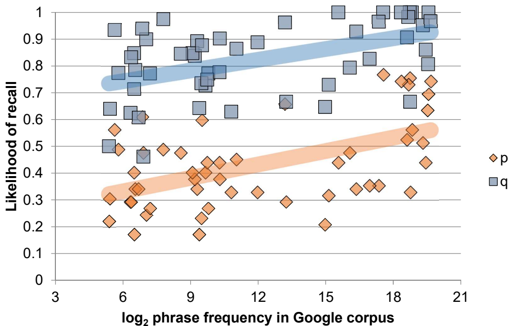
Figure 7: Effect of phrase frequency on parameters p and q in the recall of adjective-noun phrases, Google stimuli, Experiment 3. More common phrases are more likely to be recalled in whole or in part than uncommon phrases, and are more likely to be recalled in their entirety given that at least one of the words was recalled (blue squares) than less common phrases.
