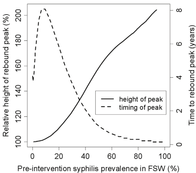
Figure 4. Timing and height of peak rebound in infectious syphilis for different FSW syphilis prevalence levels. Results are shown for model 3 using the best fit parameter set and varying \beta (transmission probability per act) between 0.01 and 1 to produce different epidemic settings. A 5-year intervention with yearly testing of all FSWs, using a rapid test of 87% sensitivity, was simulated. The x-axis shows overall pre-intervention syphilis prevalence (all infected stages) in the FSW population (high risk+low risk), and the rebound statistics shown are for infectious syphilis (primary, secondary and recurrent secondary stages) in the total FSW population (high risk+low risk). doi:10.1371/journal.pone.0055622.g004
