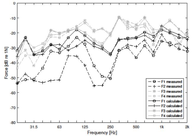
Figure 6. Measured and calculated forces.
