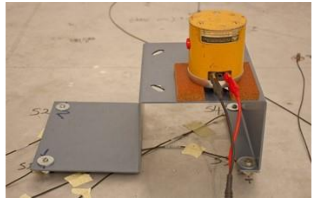
Figure 2. Test source on reception plate
