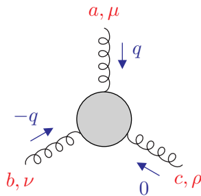
Figure 2. The triple-gluon vertex with one vanishing momentum, \Gamma_{\mu\nu\rho}^{abc}(q, -q, 0) .
