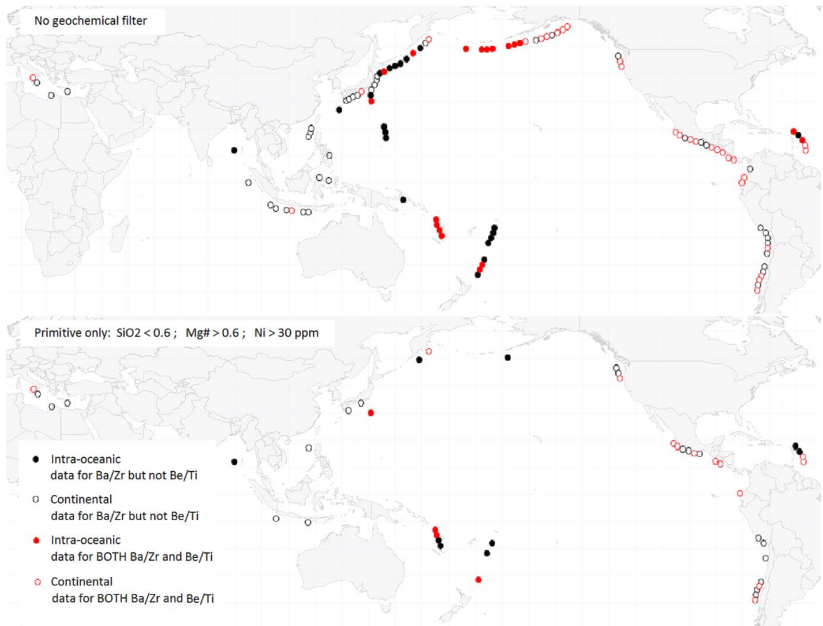
Figure 4.1 Maps of the locations of the subduction zone segments used in this study, in which each circle is a single segment. The top panel shows all the segments used for the element ratio with the most data (Ba/Zr) and for the element ratio with the least (Be/Ti). The bottom panel demonstrates which segments remain when a “primitive lava” filter is applied. Circles are either filled or empty depending on whether the over-riding plate for that segment is continental or oceanic.
