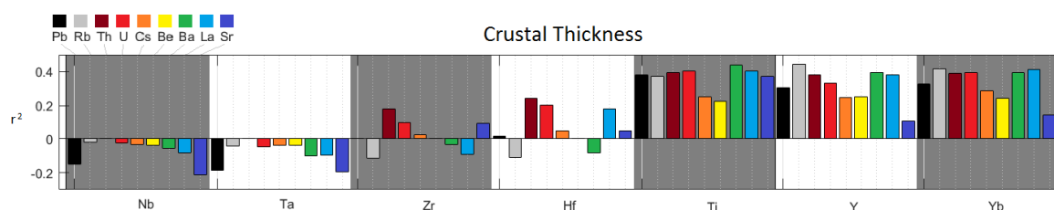
Figure 4.5 The strength of correlation ( r^2 ) of the logarithm of trace element ratios against crustal thickness. The sign of the r^2 value reflects the sense of correlation. Element ratios with the same denominator element are grouped together and numerator elements are given in the top left of each plot. All element ratios with the same numerator element have bars that are coloured the same. So, e.g., a red bar ('U') in the box named 'Nb' refers to the correlation of crustal thickness with the trace element ratio U/Nb.
