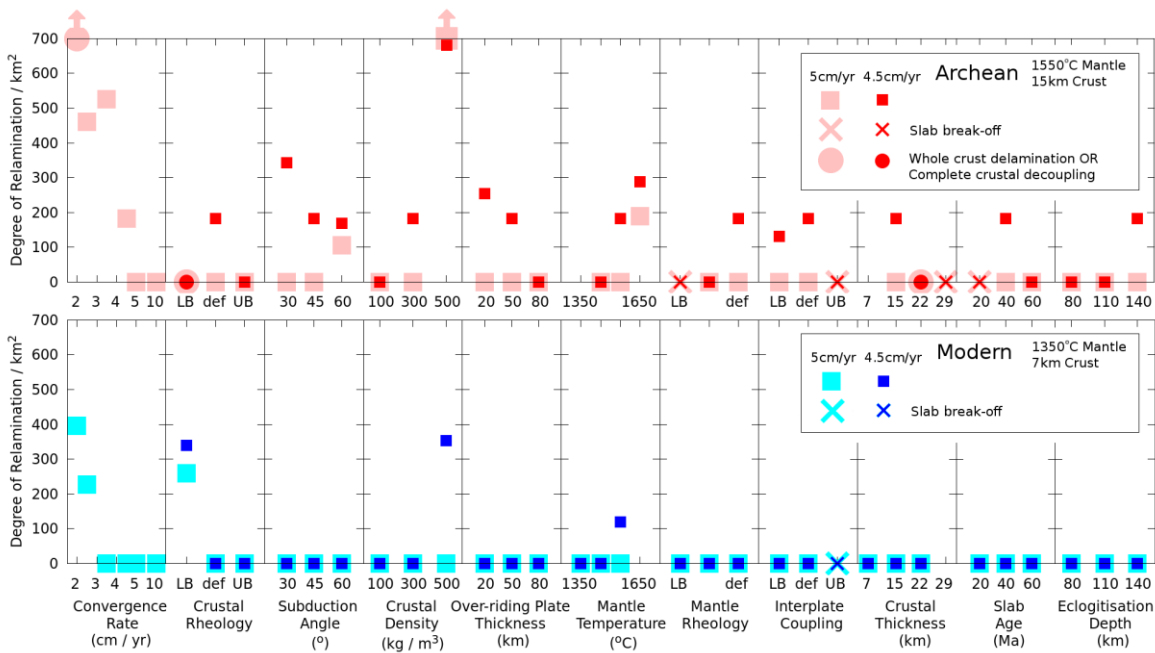
Figure 5.4 A graphical summary of the degree of relamination (see text for definition). Red symbols represent the Archean model runs and blue the modern day model runs. Darker, smaller symbols represent models where the default has a convergence rate of 4.5 cm/yr and lighter, larger symbols, 5 cm/yr. The circles represent Archean models that display relamination behaviour that is morphologically distinct from the normal “crustal plume” mode of relamination (see Section 5.3.2 and 5.3.3). Crosses represent model runs that displayed slab break off instead of subduction (see Section 5.4.3). “LB” stands for lower bound, “def” for default and “UB” for upper bound.
