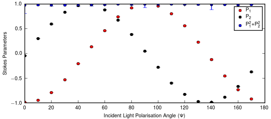
Figure 6.14: Full polarisation analysis measurements of the (1,0,0) peak at room temperature.
