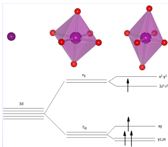
Figure 1.4: Schematic of the energy levels for a free atom, an atom in an octahedral crystal field, and an atom in a Jahn-Teller distorted Mn^{3+} octahedra.
