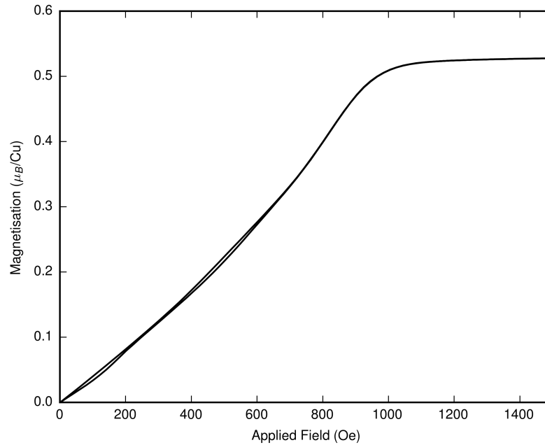
Figure 6.10: Magnetisation as a function of applied magnetic field at 20 K. The field was applied along the (1, 0, 0) direction. With a sample mass of 85.7 mg \pm 0.5.
