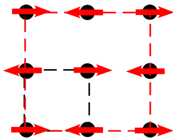
Figure 1.8: Example of how magnetism can change the unit cell size. Structural unit cell denoted by black dashed line, magnetic unit cell denoted by red dashed line.
