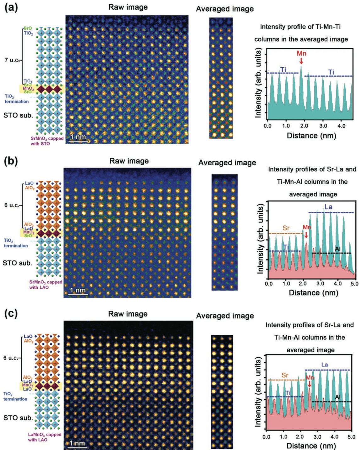
Figure 8.2: High-angle annular dark-field scanning transmission electron microscopy images with growth direction vertical for SMS (top), SML (middle) and LML (bottom). With raw image (left), averaged image (middle) and the intensity profiles (right) from [186].
