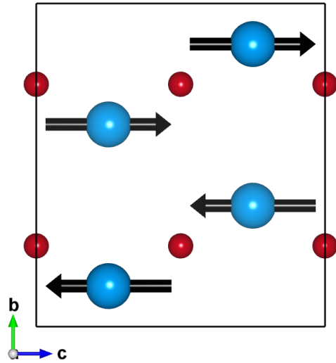
Figure 5.2: Magnetic structure of \text{CeM}_2\text{Al}_{10} ( M = \text{Fe}, \text{Os}, \text{Ru} ) with the aluminium atoms removed for clarity. Showing the cerium atoms in blue and the transition metal atoms in red
