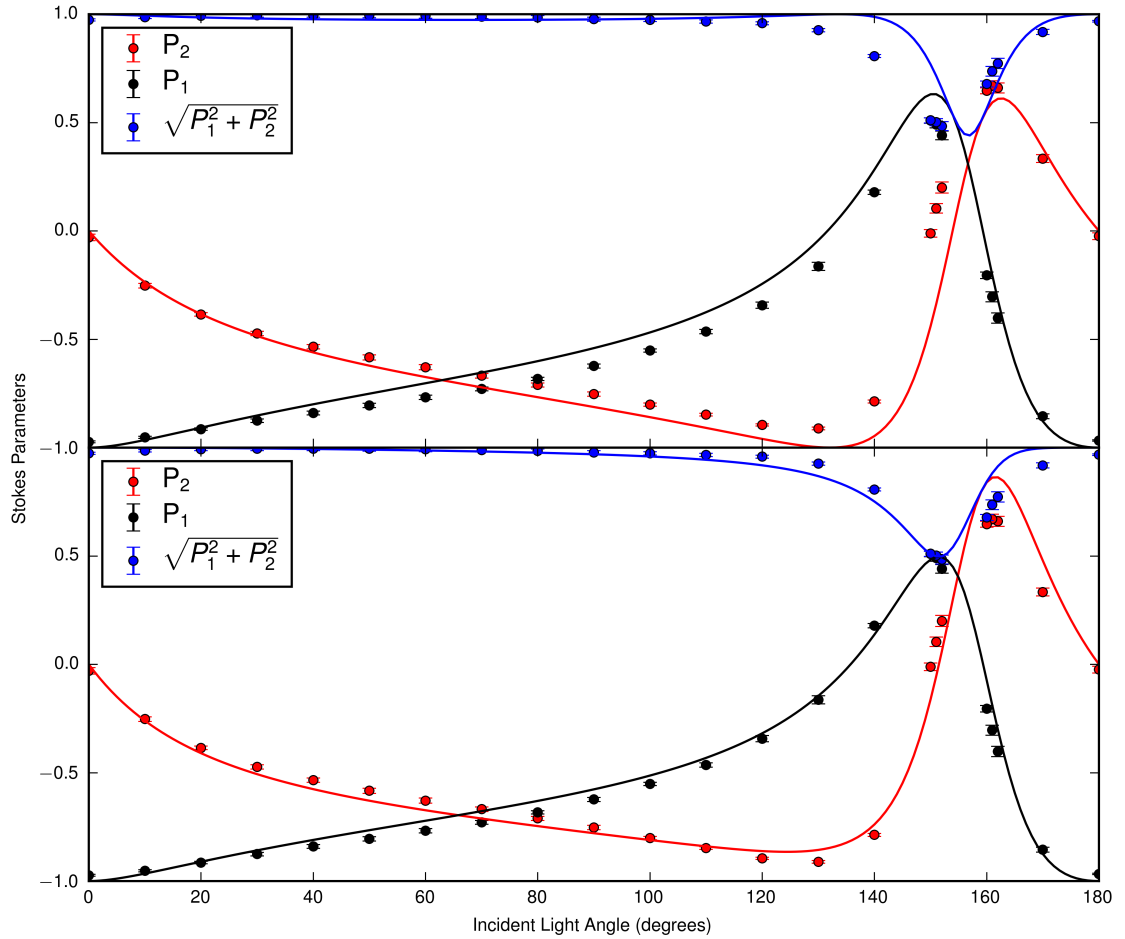
Figure 5.11: Full polarisation analysis of the (0, 1, 0) taken on resonance at 901.8 eV at 14 K. (top) Solid lines represent fits with Irreps mY_3^- and 0.15 \pm 0.007 mY_4^+ , at an azimuth of 55.01 \pm 0.35 , R^2 = 0.929 . (bottom) Solid lines represent fits with Irreps mY_3^- and 0.17 \pm 0.02 mY_3^+ , at an azimuth of 54.1 \pm 0.6 , R^2 = 0.975 .
