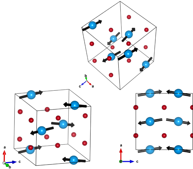
Figure 5.13: Refined magnetic structure of CeRu 2 Al 10 showing the cerium atoms in blue and the ruthenium atoms in red. The aluminium atoms have been removed for clarity.
