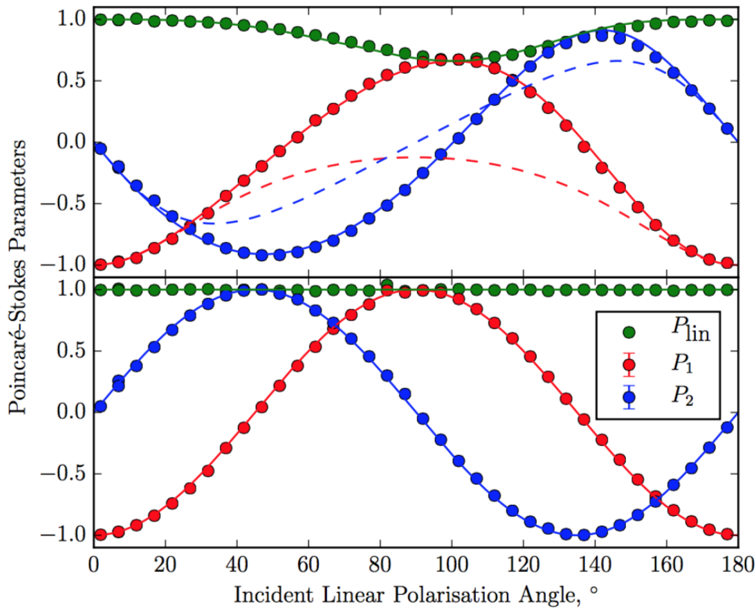
Figure 6.40: (top) Full polarisation analysis measurements of the (0, 0, \tau) reflection in FeAs at the Fe L_{III} edge. (bottom) Full polarisation analysis measurements of the (0, 0, 1 - \tau) reflection in FeAs at the Fe L_{III} edge. Figure taken from [160].
