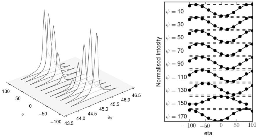
Figure 4.4: (left) Successive \theta_p scans at different \eta angles showing the change in intensity for \pi' scattered polarisation as the component of the polarisation in the scattering plane changes with the \eta angle. (right) An example of how the integrated intensity of the \theta_p scans can vary with \eta for different incident light polarisation angles \psi . These lines can be fitted to determine the P_1 and P_2 parameters.
