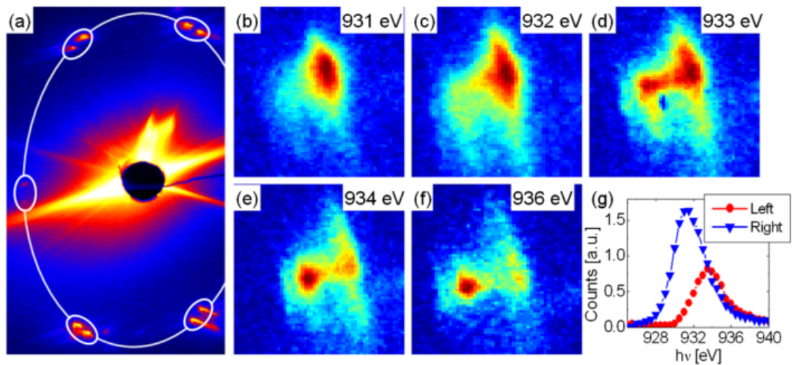
Figure 6.21: (a) Skyrmion peaks at 933 eV (b)-(f) Evolution of the double peak as a function of the incident photon energy. (g) Integrated peak intensities as a function of photon energy, showing different resonances for each peak, from [110].
