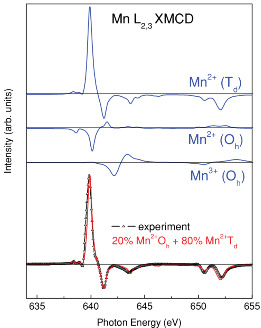
Figure 8.8: Comparison of the Mn L_{II,III} -edges' XMCD of MnFe 2 O 4 (5 nm) to the calculated Mn L_{II,III} edges XMCD for Mn 2+ ( T_d ), Mn 2+ ( O_h ), and Mn 3+ ( O_h ) (blue lines) and their weighted sum (red line) ( T = 300 K, H = 5 T) [196].
