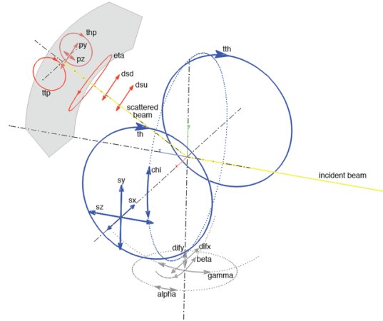
Figure 3.4: Schematic of the RASOR diffractometer [44]. With sample translations denoted s_x , s_y , s_z . Sample rotations denoted \chi and \theta . Diffractometer translations; d_{ifx} and d_{ify} , diffractometer rotations; \alpha , \beta , and \gamma . Detector angle \theta , up and down stream detector slits denoted d_{sd} and d_{su} . Polarisation analyser translations p_z and p_y . Polarisation analyser angles \eta and \theta_p and finally polarisation analyser detector angle \theta_{tp} .
