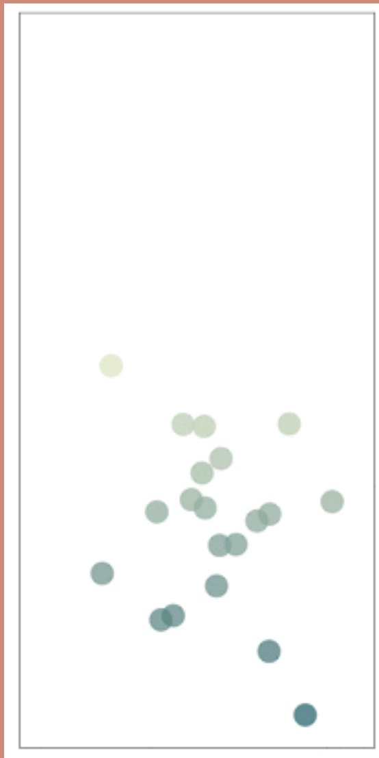
Error Accumulation
