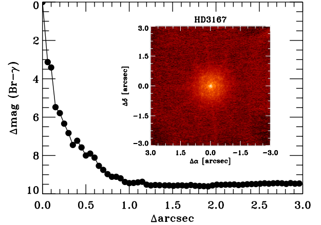
Figure 5. Keck Observatory NIRC2 K-band image and the associated contrast curve. No stars with contrasts \Delta K < 3.4 are detected with separations > 0.1 \text{ arcsec} and \Delta K < 8.0 with separations > 0.5 \text{ arcsec} .
