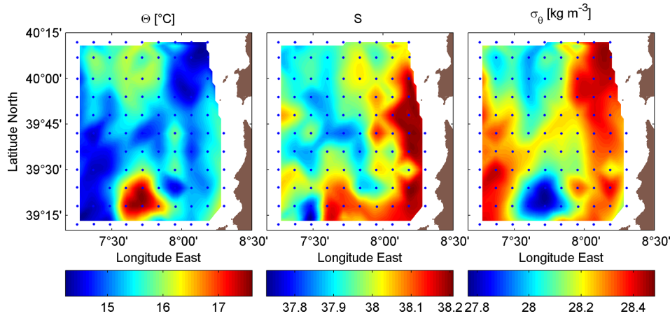
Figure 7. Potential temperature ( \Theta ), salinity ( S ), and potential density anomaly ( \sigma_{\Theta} ) distribution at the pressure level of 50 dbar based on CTD casts (blue dots) obtained by Planet from 8 to 18 June.
