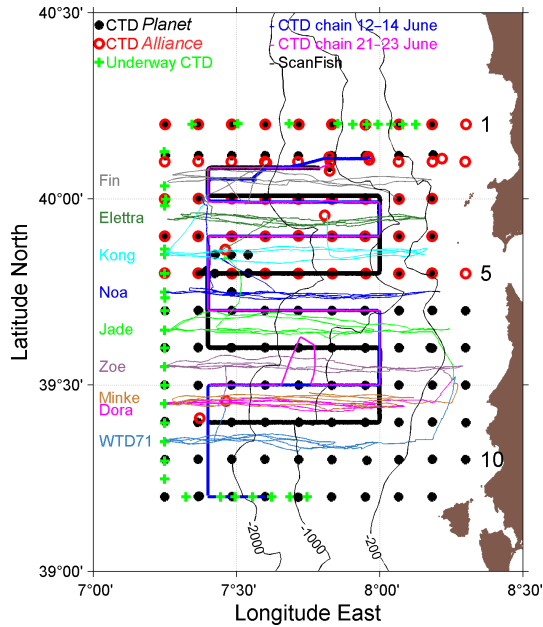
Figure 1. CTD data sets obtained with different instruments. Glider names are specified next to their tracks. For reference, zonal CTD transects 1, 5, and 10 are also marked. Thin black lines denote the 200, 1000, and 2000 m isobaths.
