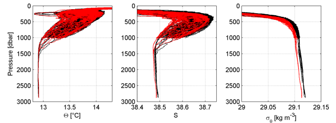
Figure 2. Potential temperature ( \Theta ), salinity ( S ), and potential density anomaly ( \sigma_\Theta ) profiles of Sea-Bird CTD casts obtained by Planet (black) and Alliance (red) with a focus on the lower water column.
