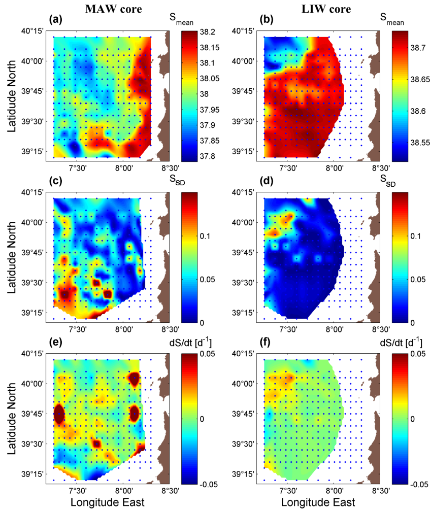
Figure 11. Mean salinity ( S_{\text{mean}} ), standard deviation ( S_{\text{SD}} ), and linear temporal change in salinity per day ( dS/dt ( \text{d}^{-1} )) in the cores of (a, c, e) MAW ( \sigma_{\Theta} = 28.2 \text{ kg m}^{-3} ) and (b, d, f) LIW ( \sigma_{\Theta} = 29.06 \text{ kg m}^{-3} ) based on all collected data of the station grid (blue dots).
