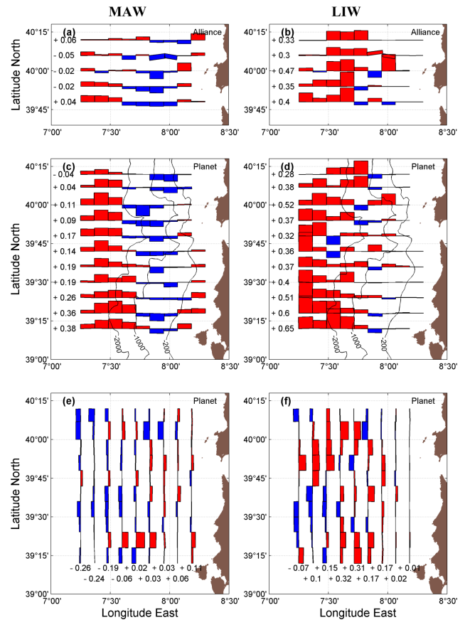
Figure 13. Geostrophic transports ( \text{Sv} ) calculated with a level of no motion (LNM) at 1000 dbar and bottom, respectively, along the CTD transects of (a, b) Alliance and (c, d, e, f) Planet within the water masses (a, c, e) MAW and (b, d, f) LIW. The net transports are noted beside each transect. Plots of the meridional transports observed by Planet additionally show the isobaths at 200, 1000, and 2000 m depth.
