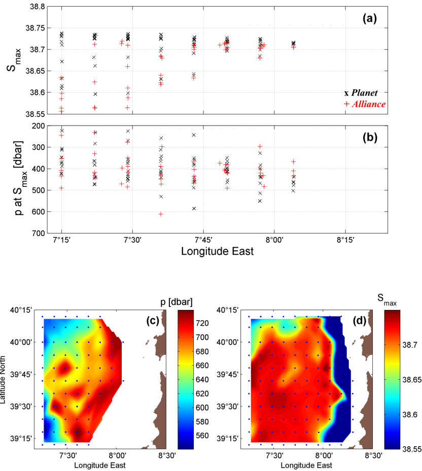
Figure 9. Characteristics of LIW, (a) salinity maximum ( S_{\max} ) of at least 400 dbar deep CTD casts of Planet (x) and Alliance (+), (b) corresponding pressure level of S_{\max} , (c) pressure level of lower boundary of LIW ( \sigma_{\Theta} = 29.1 \text{ kg m}^{-3} ) based on Planet CTD casts (blue dots), and (d) maximum salinity ( S_{\max} ) > 38.55 based on Planet CTD casts (blue dots).
