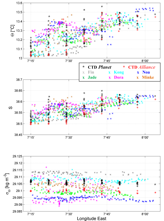
Figure 3. Potential temperature ( \Theta ), salinity ( S ), and potential density anomaly ( \sigma_\Theta ) at roughly 900 dbar versus longitude of all CTD and glider profiles available at that pressure level. Planet covered all latitudes of the trial area, Alliance observed in the northern part, and the gliders surveyed at selected latitudes given in Fig. 1.
