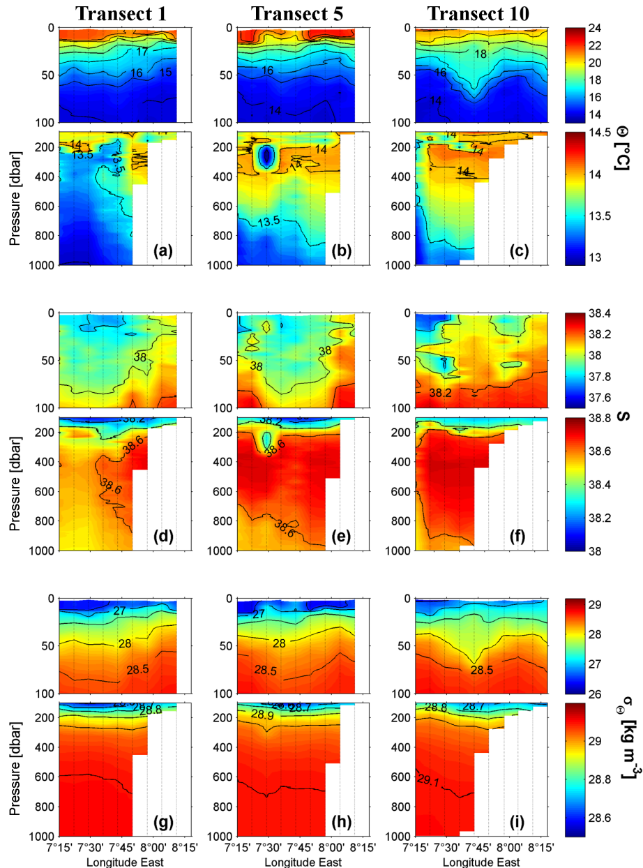
Figure 5. Potential temperature ( \Theta ), salinity ( S ), and potential density anomaly ( \sigma_{\Theta} ) along the zonal (a, d, g) transect 1 ( 40^{\circ}12'N ), (b, e, h) transect 5 ( 39^{\circ}48'N ), and (c, f, i) transect 10 ( 39^{\circ}18'N ) in the upper 100 and 1000 dbar based on Planet CTD casts (dotted lines) given in Fig. 1.
