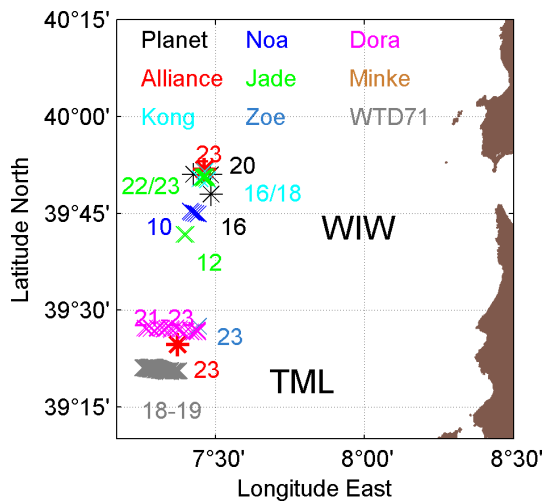
Figure 8. Positions (symbols) and June dates (numbers) of all CTD and glider profiles with WIW and TML observations, respectively ( T < 13.3^{\circ}\text{C} and S < 38.33 between 100 and 350 dbar).
