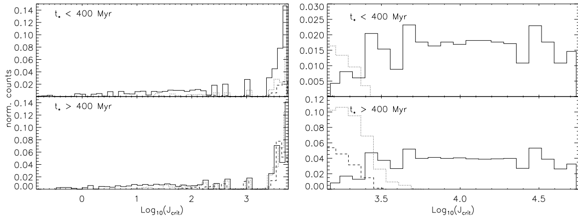
Figure B2. Histograms of J_{crit} for the ISb model, IB (left panel) and the CSf model, CB (right panel). The histograms are plotted by splitting the stellar populations into ones with t_* > 400 Myr and t_* < 400 Myr. The values of J_{crit} are obtained by requiring that Eq. 17 be valid in the grey regions in Fig. 3. The solid, dotted and dashed lines correspond to the 5, 12 and 20 kpc separations respectively.
