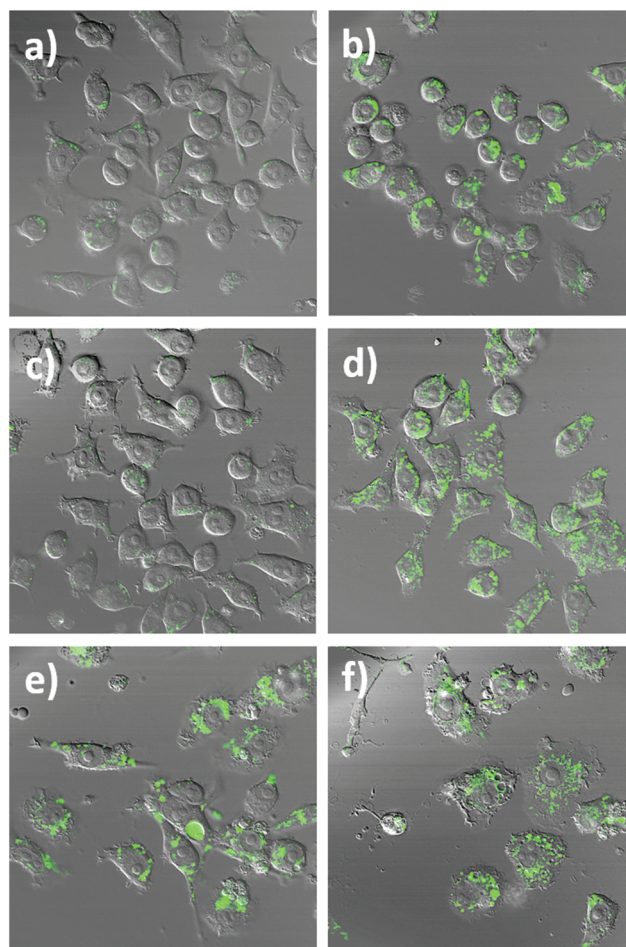
Fig. 4 Confocal fluorescence microscopy images of RAW264.7 NO - cells incubated with the NO nanobiosensor (10 nM) under different conditions: (a and b) control, (c and d) INF- \gamma (10 ng mL -1 ) only, and (e and f) INF- \gamma (10 ng mL -1 ) and LPS (500 ng mL -1 ) before (a, c and e) and after (b, d and f) the addition of the NO donor SNAP (100 \mu\text{M} ). The green fluorescence is due to the emission of the NO nanobiosensor upon excitation at 488 nm (emission collected between 505–545 nm). Images (a)–(f) are composite images of the green and DIC channels.
