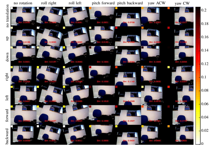
Fig. 7: Predicted images for active SLAM with their divergence distance with respect to the current image. Divergence values are also depicted with color-coded patches on top-left corner of each predicted image. The color bar (right) shows the divergence values.
