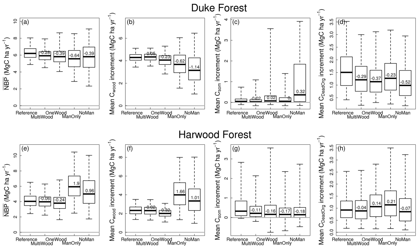
Figure 2. Box and whisker plots show the median and distribution information retrieved for (a, e) the mean annual net biome productivity (NBP), and the mean annual accumulation of (b, f) C_{wood} , (c, g) C_{som} , and (d, h) C_{DeadOrg} . A positive value indicates a net accumulation of carbon within the forest or carbon pool. The median is shown by the thick black horizontal line, while the box and whiskers represent the 50% and 95% confidence intervals, respectively. The number imposed on each graph is the bias between the Reference analysis and the respective data availability scenario. Figures 2a–2d are Duke Forest, and Figures 2e–2h are Harwood Forest.
