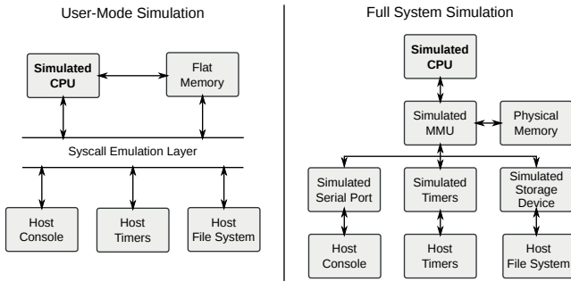
Fig. 1: User-Mode simulation with a simple memory model supporting one virtual address space and syscall emulation vs. Full-System simulation – capable of hosting a full OS – with a simulated MMU and I/O devices backed by host counterparts.
