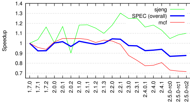
Fig. 2: Relative performance of the sjeng and mcf benchmarks and the overall SPEC rating (weighted geometric mean across all benchmarks) on a variety of QEMU versions for x86. Version 1.7 is used as a baseline.
