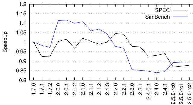
Fig. 8: Graph of geometric mean of speedup of QEMU (baseline is v1.7.0) running SPEC2006 Integer benchmarks, and SimBench, across a range of QEMU versions.
