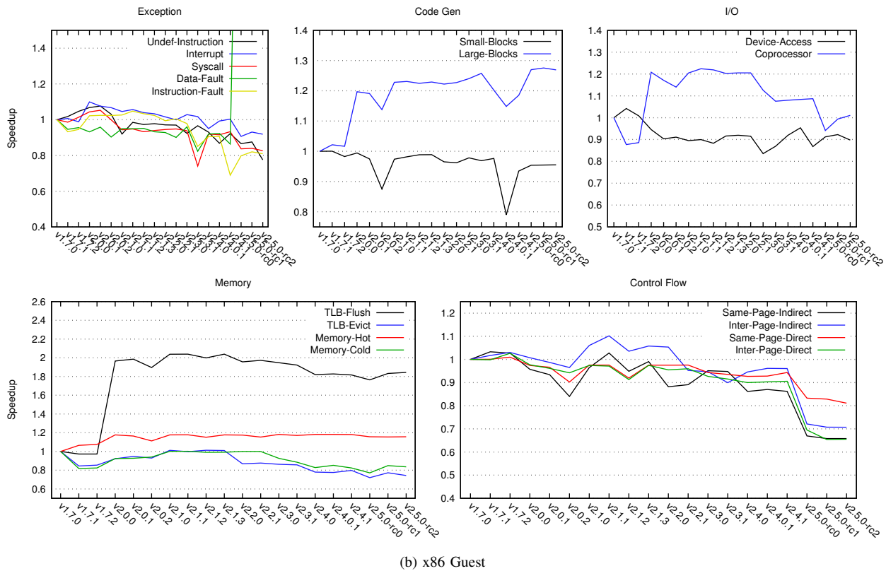
Fig. 6: Graphs showing the performance of the QEMU-DBT simulator on each category of the SimBench benchmarks. For the Data-Fault Exception benchmark we observed a speedup of around 8x on ARM and 4x on x86 for the 2.5.0 versions of QEMU-DBT (result which is off the scale on the corresponding graphs). The host (an HP z440 workstation) is specified in Figure 5.
