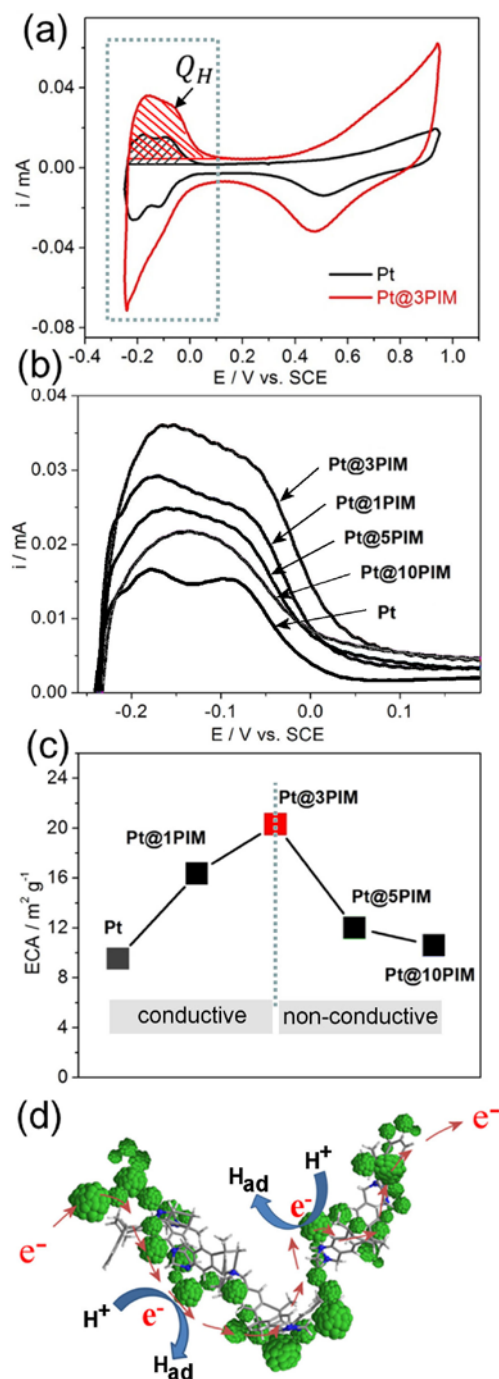
Figure 5. (a) Cyclic voltammograms (scan rate 0.05 Vs -1 ) for Pt and Pt@3PIM immersed in 0.1 M HClO 4 . (b) Hydrogen adsorption region within cyclic voltammograms for different samples. (c) Electrochemically active surface area (ECA) versus Pt@PIM sample. (d) Schematic mechanism of hydrogen adsorption/desorption in PIM-EA-TB stabilized Pt coupled to electrical conductivity.
