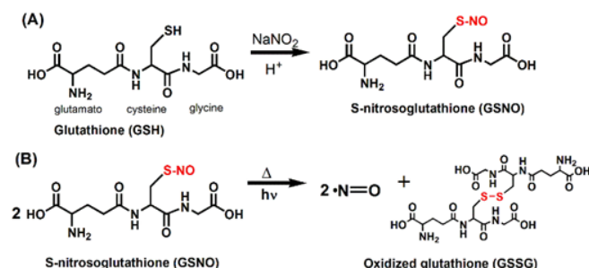
Figure 2. Nitrosation of glutathione (GSH) by sodium nitrite ( \text{NaNO}_2 ) yielding S-nitrosoglutathione (GSNO) (A), which thermally or photochemically releases free NO (B).
