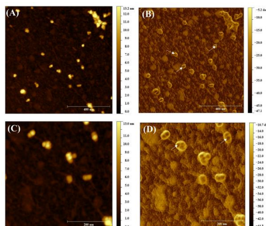
Figure 1. AFM topographic (left) and phase contrast (right) images of GSH-CS NPs (GSH concentration of 100 \text{ mmol L}^{-1} ).
