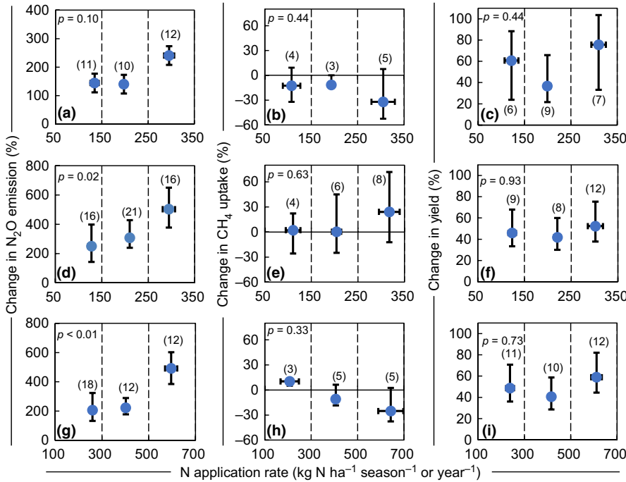
FIGURE 3 Effect of mineral N application rate on \text{N}_2\text{O} emission, \text{CH}_4 uptake, and yield relative to no N fertilizer application for (a–c) wheat season, (d–f) maize season, and (g–i) annual period. Horizontal error bars represent standard errors which reflect distribution of N application rate for each N level. Error bars in vertical directions represent 95% confidence intervals of the percentage changes. Figures in parentheses indicate the number of observations
