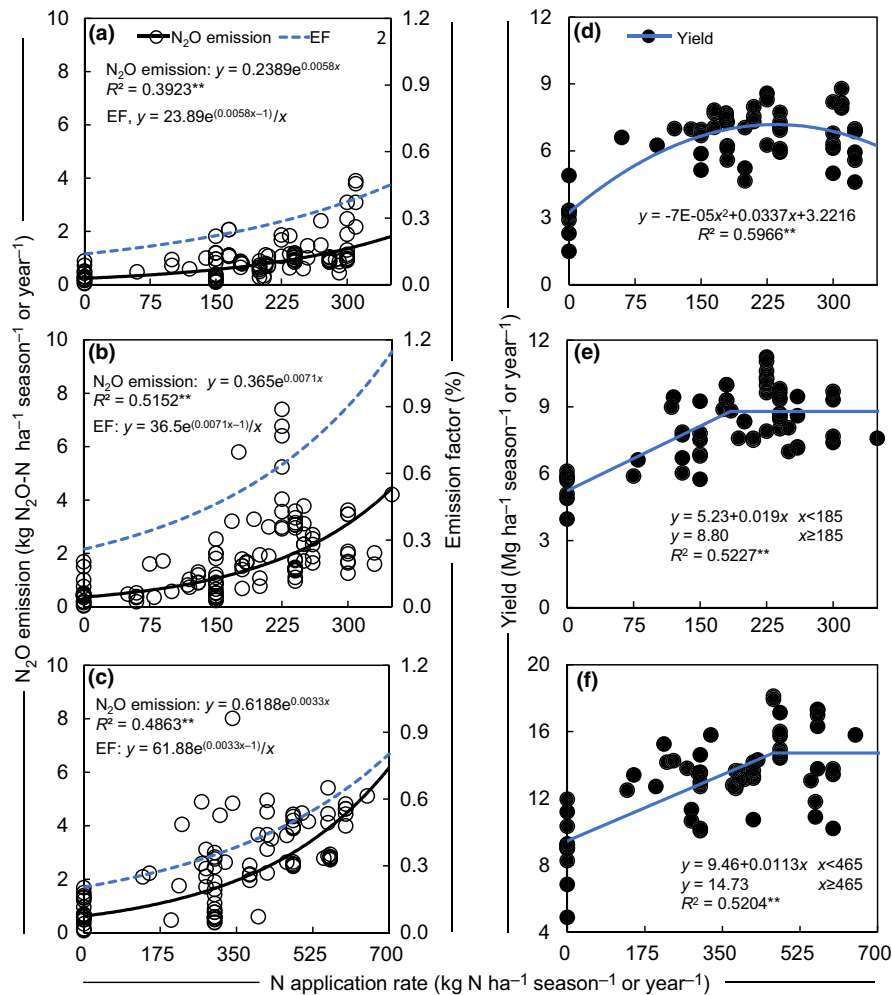
FIGURE 4 \text{N}_2\text{O} emission and emission factor (EF) versus N application rate for (a) wheat season, (b) maize season, and (c) annual period, and yield versus N application rate for (d) wheat season, (e) maize season, and (f) annual period. EF curves were generated from regression models of \text{N}_2\text{O} emission with N application rate. ** represents .01 significance level.
