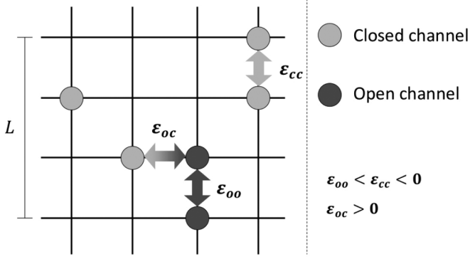
FIG. 1. Diagram representing the lattice model. Channels interact with nearest neighbors with energies \varepsilon_{oo} , \varepsilon_{cc} , and \varepsilon_{oc} , depending on the states of the interacting channels.
