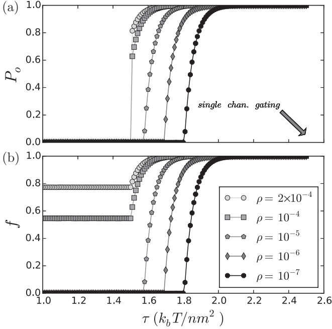
FIG. 2. Fraction of open channels in the system, P_o (a), and fraction of channels that belong to the cluster, f (b), as functions of the membrane tension \tau , for different values of \rho . Here \varepsilon_{oo} = -15.0 k_B T , \varepsilon_{cc} = -5.0 k_B T , and \varepsilon_{oc} = 10.0 k_B T .
