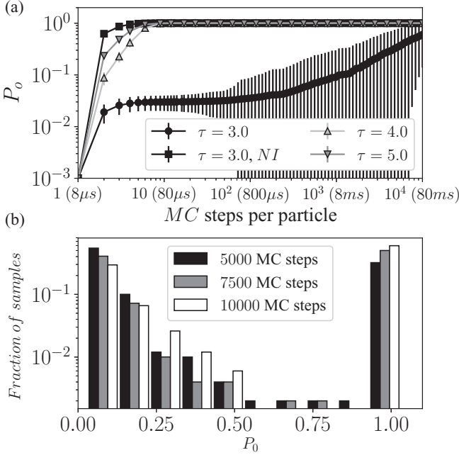
FIG. 3. (a) Average fraction of open channels as a function of simulated time, for different values of \tau . Black squares represent the same system without interaction between channels. Real time is shown in parentheses on the x axis. (b) Number of samples with a given fraction of open channels, for three different transients, for the interacting case with \tau = 3.0 k_B T / \text{nm}^2 . The parameters are \lambda_D / \lambda_G = 0.02 , L = 400 , \rho = 0.002 , \varepsilon_{oo} = -15.0 k_B T , \varepsilon_{cc} = -5.0 k_B T , and \varepsilon_{oc} = 10.0 k_B T . For each set of parameters, 500 samples were considered, and error bars correspond to one standard deviation.
