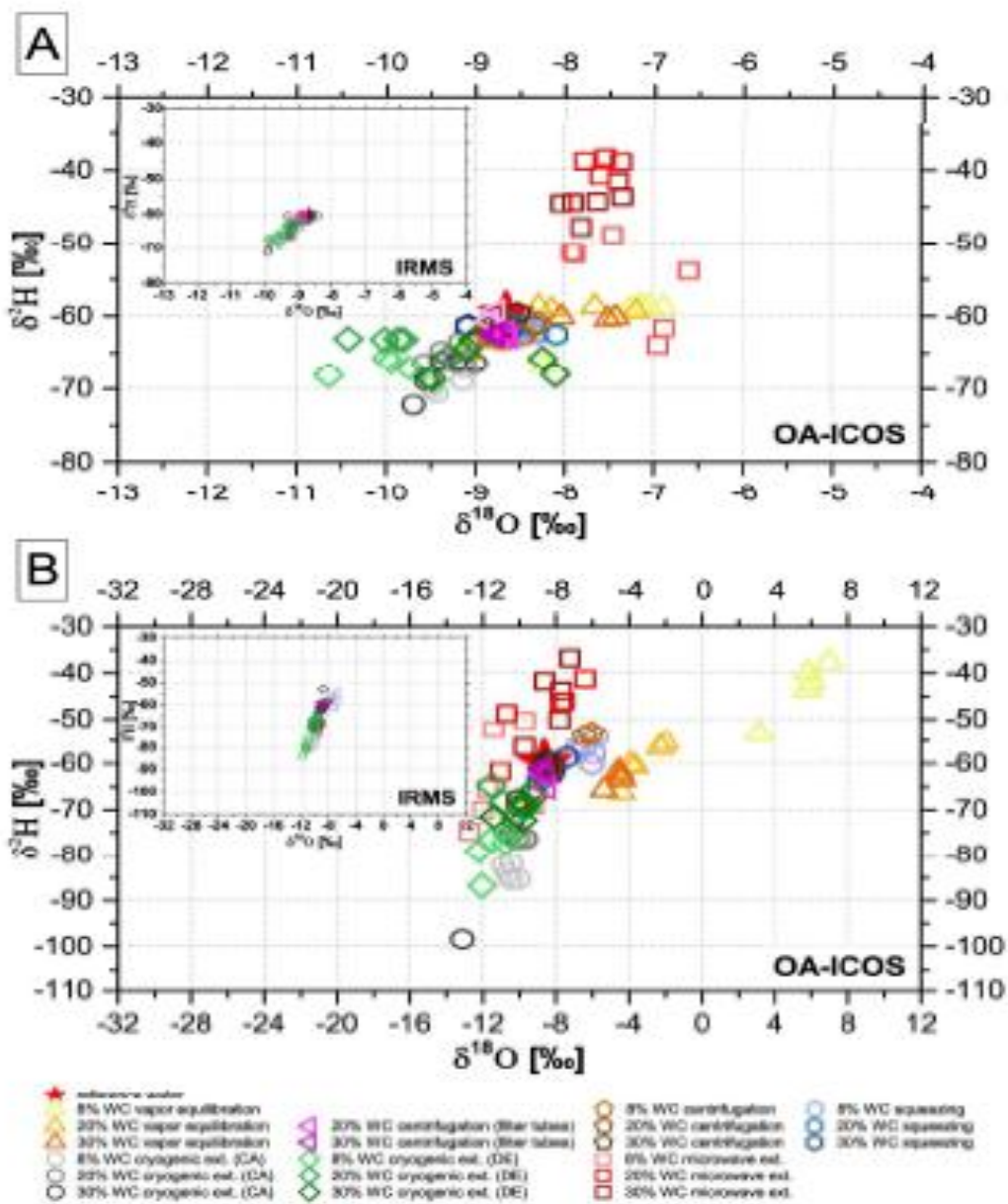
Figure 3. Dual isotope plots for silty sand (A) and clayey loam (B) water extracts of all methods and water contents (WC) in comparison to the reference water (red asterisk) for OA-ICOS and IRMS measurements (insets upper left).
