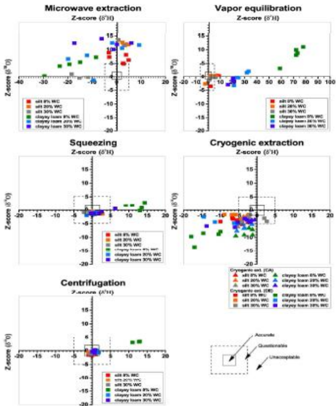
Figure 2. Performance cross plot of \delta^2\text{H} and \delta^{18}\text{O} Z-scores measured via OA-ICOS for all extraction methods, both soil types, and water contents (WC).
