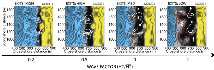
Fig. 16. Synthesis of flow behaviours from validated XBeach model simulations over measured bathymetry at Perranporth Beach in the UK showing how wave forcing ( H_s T_p / \overline{H_s T_p} ) can control circulation regime over a rip-channelled morphology (adapted from Scott et al., 2014). Greyscale is wave dissipation from high (black) to low (light grey).
