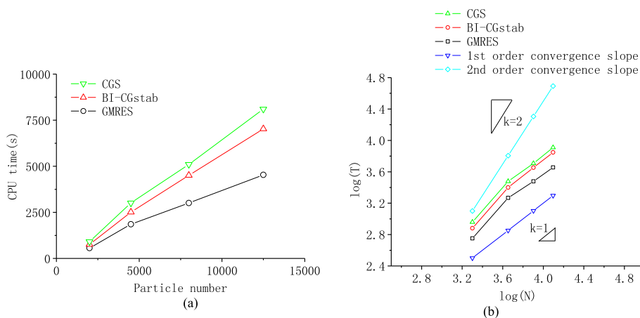
Fig. 15. Comparison of CPU time for violent water sloshing simulation by different iteration methods: (a) CPU time comparison, (b) Convergence slope comparison.
