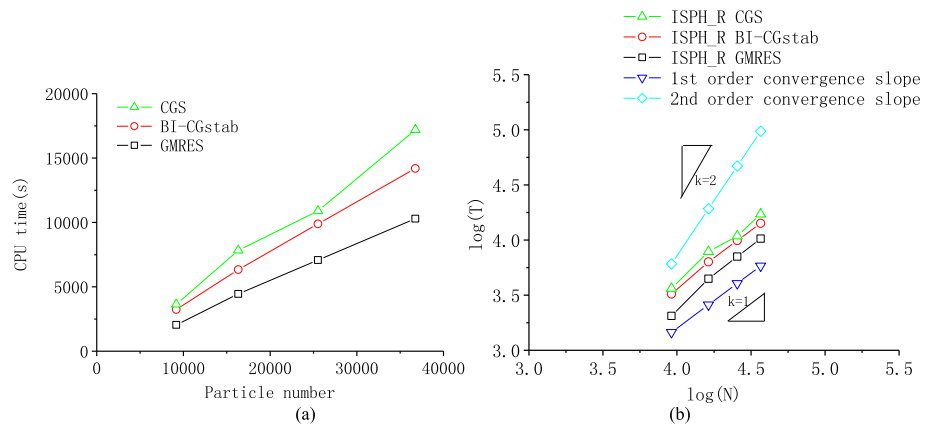
Fig. 20. Comparison of CPU time for solitary wave slamming by different iteration methods: (a) CPU-time comparison; (b) Convergence-rate comparison.
