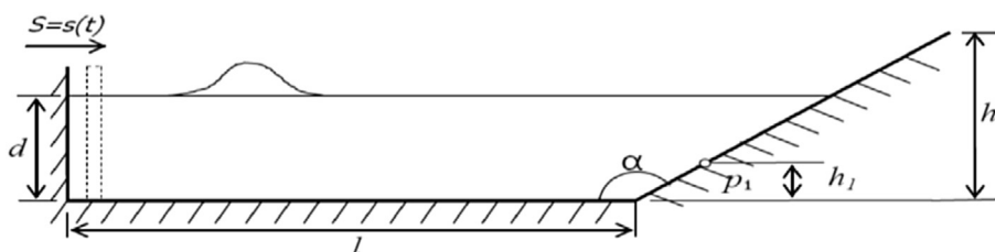
Fig. 16. The model of wave tank for solitary wave slamming.
