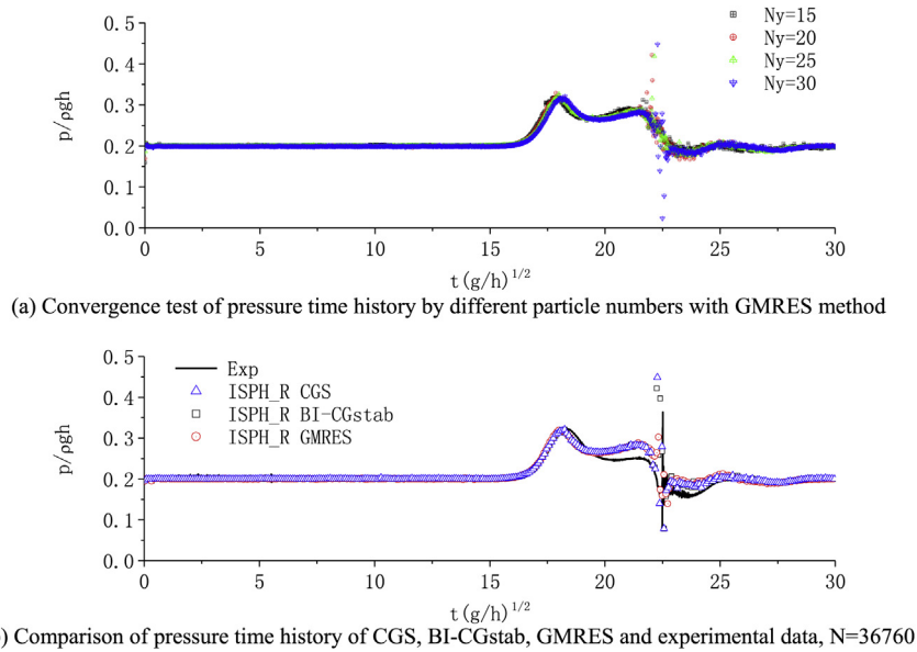
Fig. 19. Comparison of pressure time history of ISPH_R by different iteration methods for solitary wave slamming.
