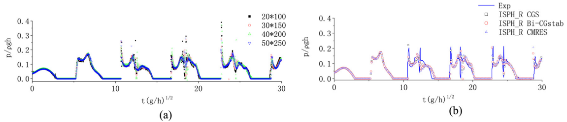
Fig. 14. Comparison of pressure time history of ISPH_R by different iteration methods for violent sloshing simulation: (a) Convergence test of pressure time history by different particle numbers with GMRES method; (b) Comparison of pressure time history of CGS, Bi-CGstab, GMRES and experimental data, N = 50*250 .
