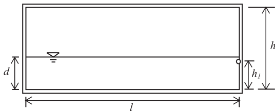
Fig. 11. Sketch of sloshing tank.
