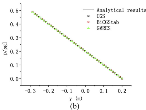
Fig. 3. Pressure distribution by different iteration methods when tolerances error RTOL = 10e-6 : a) Total pressure distribution N_y = 40 ; b) Comparison of different iteration methods when x = 0.5 m.
