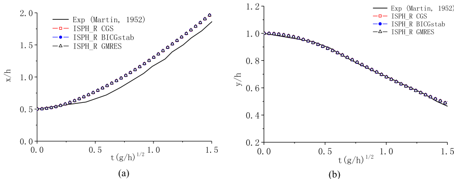
Fig. 6. Comparison of different iteration methods with experimental results: (a) wave front on the bottom wall (b) wave height on vertical wall.
