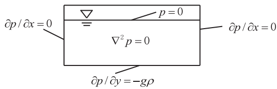
Fig. 1. Calculation domain and its boundary conditions.
