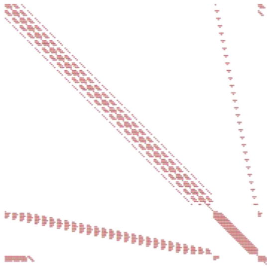
Fig. 2. Matrix elements distribution of ISPH_R (* = non-zero element, blank space = zero element, total particle number = 10*20).
