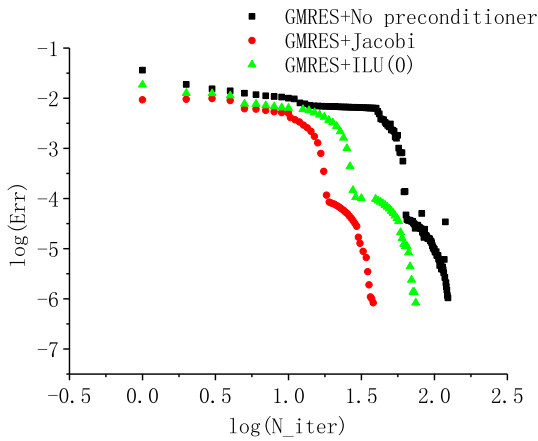
Fig. 4. Pressure distribution by different iteration methods when tolerances error RTOL = 10e-6 .
