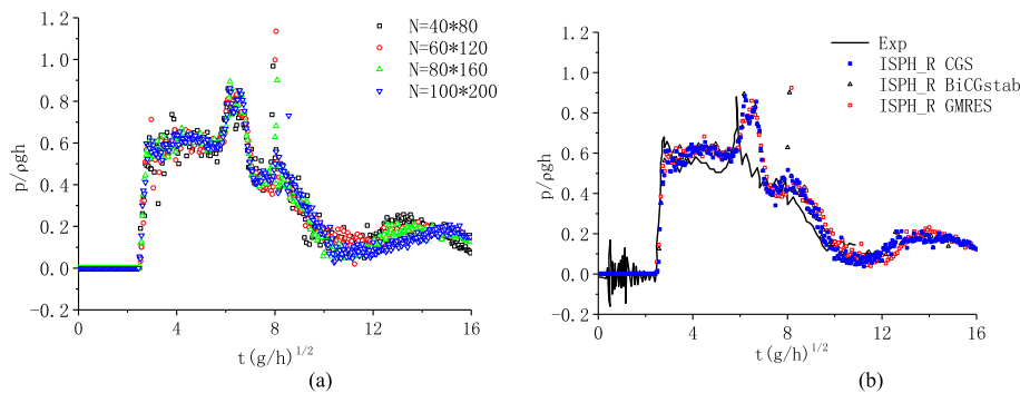
Fig. 9. Comparison of pressure time history of ISPH_R by different iteration methods: (a) Convergence test of different particle numbers by GMRES; (b) Comparison of CGS, Bi-CGstab, GMRES and experimental data, N = 100 \times 200 .
