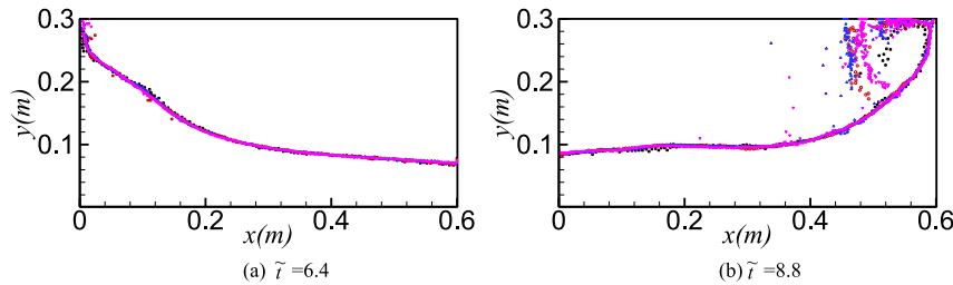
Fig. 13. Convergence test of free surface profile by GMRES method for violent water sloshing: \circ N = 20*100 , \square N = 30*150 ; \triangle N = 40*200 ; \nabla N = 50*250 .
