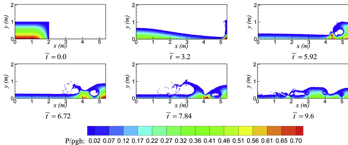
Fig. 7. Snapshot of wave profile and pressure distribution of dam breaking at different time.
