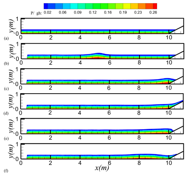
Fig. 17. Snapshots of profile and pressure distribution for solitary wave slamming of different time: (a) \tilde{t}=0.0 ; (b) \tilde{t}=10.5 ; (c) \tilde{t}=18 ; (d) \tilde{t}=20.4 ; (e) \tilde{t}=22.5 ; (f) \tilde{t}=24.0
