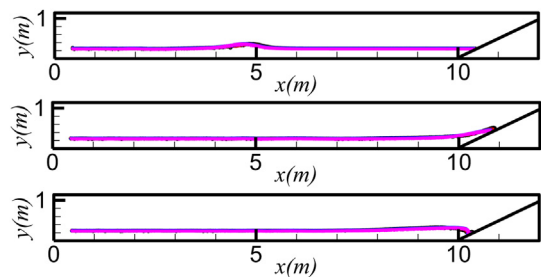
Fig. 18. Convergence test of free surface profile by GMRES method for solitary wave slamming: \circ N = 9185 , \square N = 16333 ; \triangle N = 25525 ; \nabla N = 36760 .
