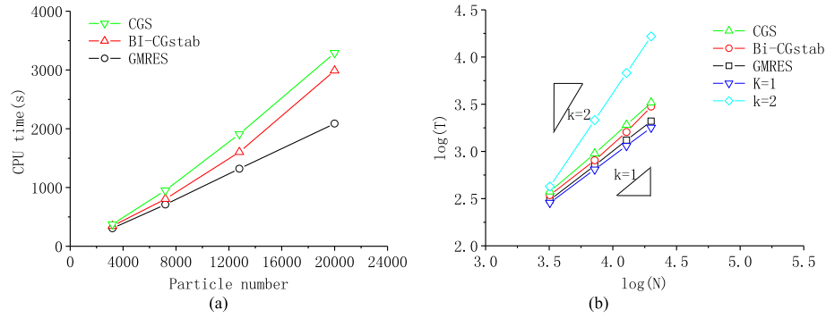
Fig. 10. Comparison of CPU time for dambreaking simulation by using different iteration methods: (a) CPU-time comparison, (b) Convergence-rate comparison.
