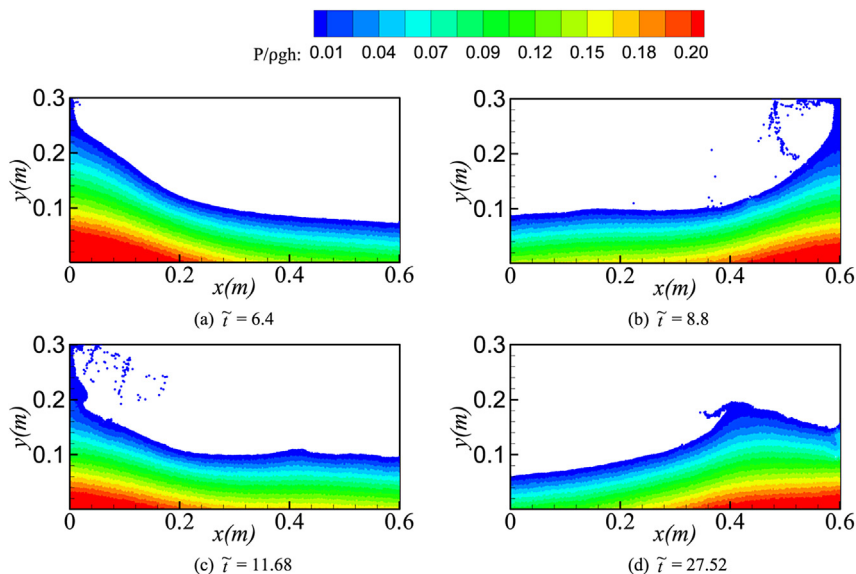
Fig. 12. Wave profiles and compress distribution of different time by GMRES method when N = 50*250 .
