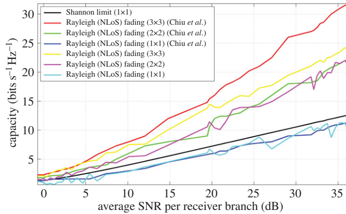
Figure 6. Simulated capacity of uni-polarized, dual-polarized and tri-orthogonal arrangements at 2.55 GHz, in a Rayleigh (NLoS) fading channel, and as a function of average SNR per receiver branch at the FoV centre, according to prior work [11]. A Ricean factor K of 10^{-2} is used. The transmitter is perfectly aligned with the receiver along the positive C axis, as in figure 3. The difference in capacity between the tri-orthogonal, or 3 \times 3 , arrangement of the presented model and the simulated and measured 3 \times 3 arrangement in the work of Chiu et al. is due to a non-orthogonal arrangement at the transmitter being previously employed.
