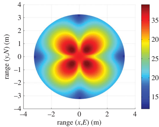
Figure 9. Tri-orthogonal, or 3 \times 3 , AWGN fading channel capacity ( \text{bits s}^{-1} \text{Hz}^{-1} ).
