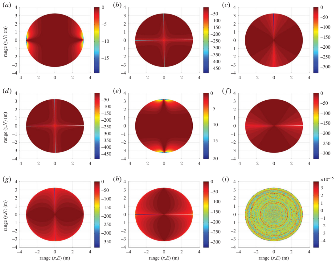
Figure 5. Polarization mismatch ( e_{\text{pol}} ) (dB) profiles for each unit dipole pair: (a) \hat{x}\hat{p} , (b) \hat{y}\hat{p} , (c) \hat{z}\hat{p} , (d) \hat{x}\hat{q} , (e) \hat{y}\hat{q} , (f) \hat{z}\hat{q} , (g) \hat{x}\hat{r} , (h) \hat{y}\hat{r} and (i) \hat{z}\hat{r} .
