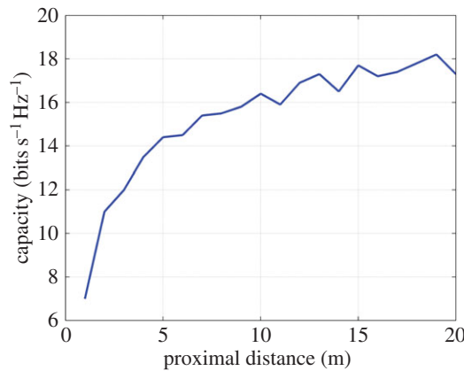
Figure 15. Capacity advantage (bits s -1 Hz -1 ) of a rich scattering environment such as a Rayleigh fading channel over that of an AWGN fading channel. The proximal distance is shown in figure 2 as d .
