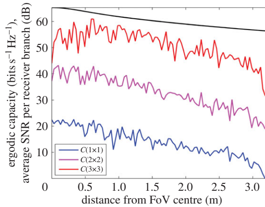
Figure 14. Rayleigh fading channel capacity (bits s -1 Hz -1 ) profile at \theta_T = 90^\circ for uni-polarized, dual-polarized and tri-orthogonal systems. The average SNR per receiver branch as a function of distance from the FoV centre is also shown.
