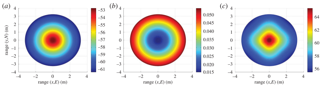
Figure 8. (a) Free space path loss (dB), (b) atmospheric loss L_{\text{atmos}} (dB) and (c) average SNR per receiver branch for a tri-orthogonal system (dB) profiles over the FoV.
