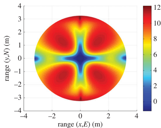
Figure 10. Capacity advantage ( \text{bits s}^{-1} \text{Hz}^{-1} ) of a tri-orthogonal, or 3 \times 3 , system over that of a dual-polarized, or 2 \times 2 , system in an AWGN fading channel.
