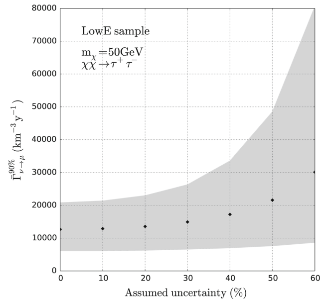
Fig. 4 Effect of the assumed uncertainty on the sensitivity of the volumetric flux. The example shows 50 GeV WIMPs annihilating into \tau^+ \tau^- . The points show the estimated sensitivity and include a correction for coincident muons, while the band indicates one standard deviation
