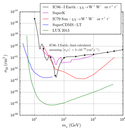
Fig. 8 Upper limits at 90% confidence level on \sigma_{\chi-N}^{SI} as a function of the WIMP mass assuming a WIMP annihilation cross section of \langle\sigma_A v\rangle = 3 \times 10^{-26} cm^3 s^{-1} . For WIMP masses above the rest mass of the W bosons, annihilation into W^+W^- is assumed and annihilation into \tau^+\tau^- for lower masses. Systematic uncertainties are included. The result is compared to the limits set by SuperCDMSlite [6], LUX [5], Super-K [22] and by a Solar WIMP analysis of IceCube in the 79-string configuration [24]. The displayed limits are assuming a local dark matter density of \rho_\chi = 0.3 GeV cm^{-3} . A larger density, as suggested e.g. by [59], would scale all limits linearly
