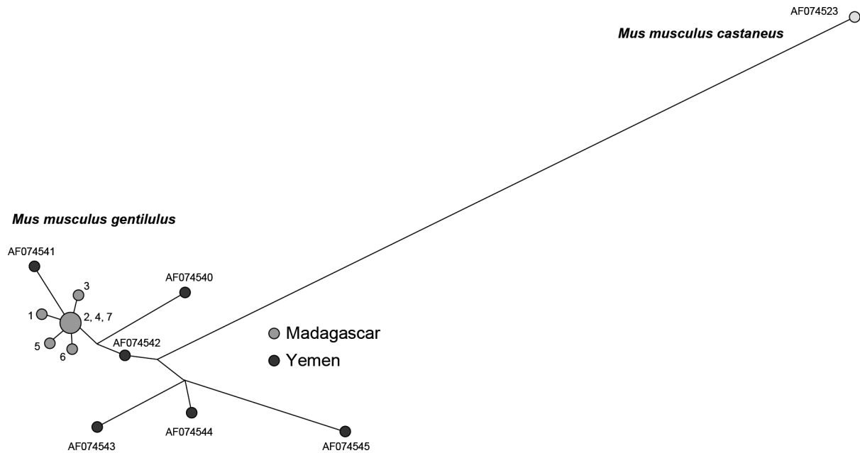
Fig. 4. A network for mitochondrial control region with sequences (539 bp) from Madagascar mice (specimen code Nos. 1–7) and those from databases for mice from Yemen or of Mus musculus castaneus . The codes associated with haplotypes represent accession numbers.
