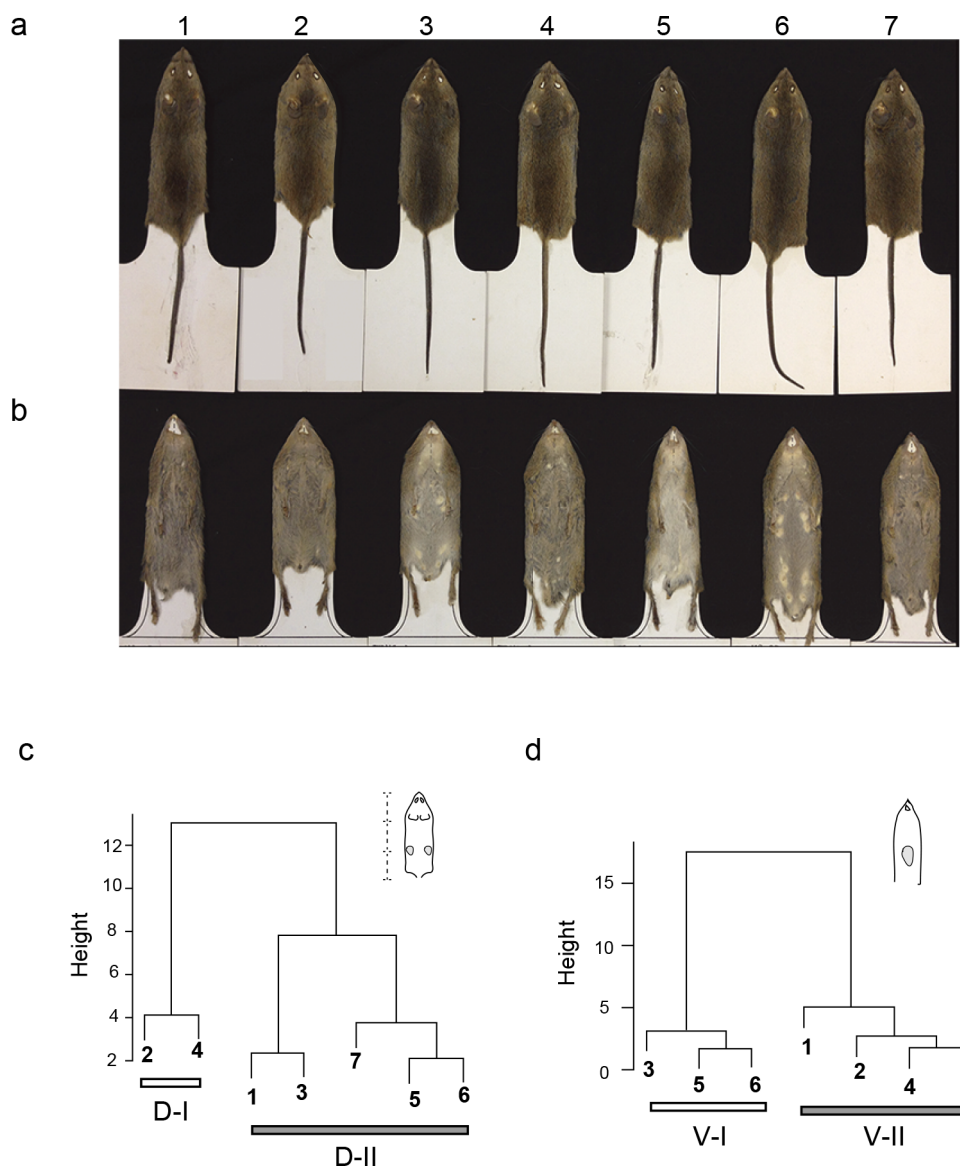
Fig. 3. Images showing coat color variations on dorsal (a) and ventral (b) sides in the seven Madagascar mice (specimen code Nos. 1–7 in Table 1) used in this study. Dendrograms based on spectrophotometer measurements revealed the color types on dorsal (c) and ventral (d) sides. Shaded areas in the flat skin specimens represent the regions used for color measurements.
