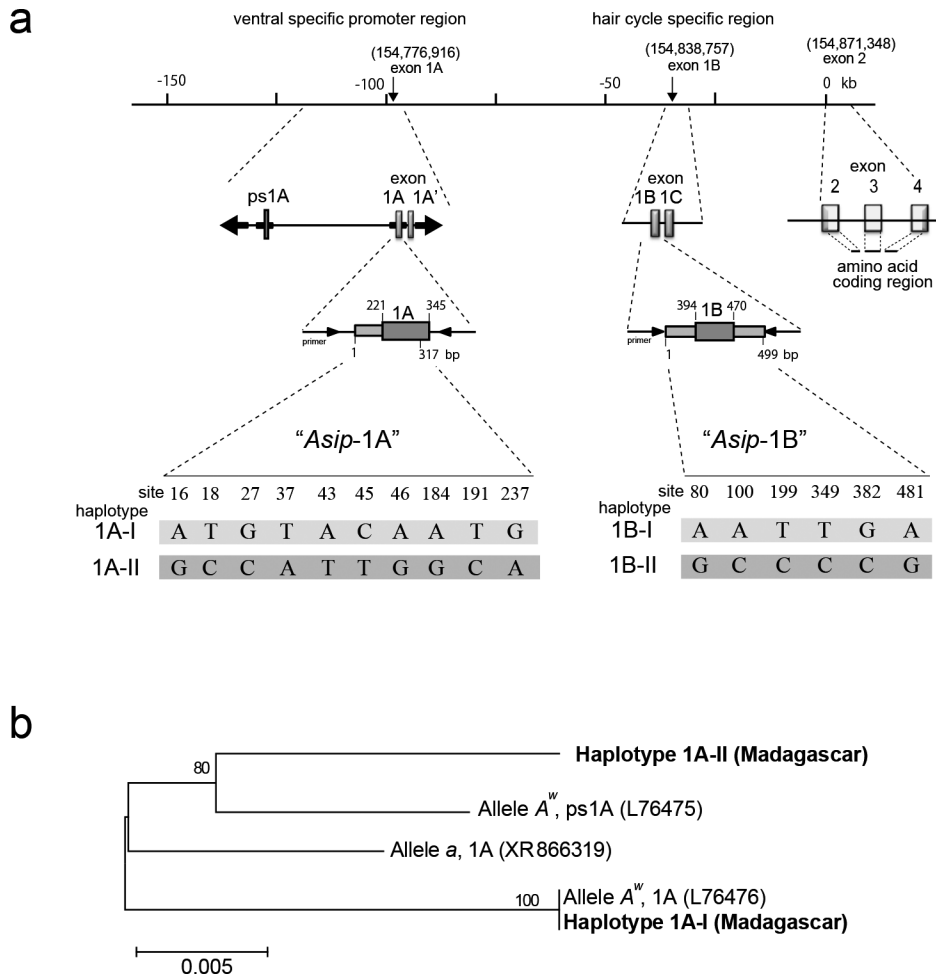
Fig. 2. A schematic representation of the coat color-related gene, Asip (Vrieling et al. 1994) (a). The two exon-1-associated promoter regions are indicated (1A-1A' and 1B-1C). The thick arrows indicate the inverted repeats, one of which carries the pseudo promoter, termed ps1A (Chen et al. 1996). The two amplified regions, Asip -1A (317 bp) and Asip -1B (499 bp), are indicated by the filled boxes. The chromosomal locations for the starting sites of exon 1A, 1B, and 2 are shown in parentheses and refer to the mouse genome sequence of chromosome 2 (strain C57BL/6J, NCBI build 37/mm9 http://genome.ucsc.edu ). Two haplotypes recovered from the analyses of the sequenced regions are shown with the variable sites detected. An ML tree was constructed using the sequences of Asip -1A (317 bp) and three database sequences for the 1A and ps1A regions of allele A^w , and the 1A region of allele a (Vrieling et al. 1994) (b). Bootstrap support values (>50%) are shown at the nodes and are based on 1,000 resampling replicates.
