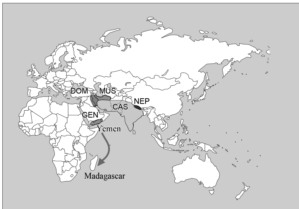
Fig. 1. A map of the Madagascar collection sites. The predicted homeland areas of the five major mitochondrial lineages of Mus musculus , M. m. castaneus (CAS), M. m. domesticus (DOM), M. m. gentilulus (GEN), M. m. musculus (MUS), as well as mice from Nepal (NEP) are shown. The Madagascar mitochondrial lineage is thought to be derived from GEN mice introduced from Yemen (Duplantier et al. 2002).
