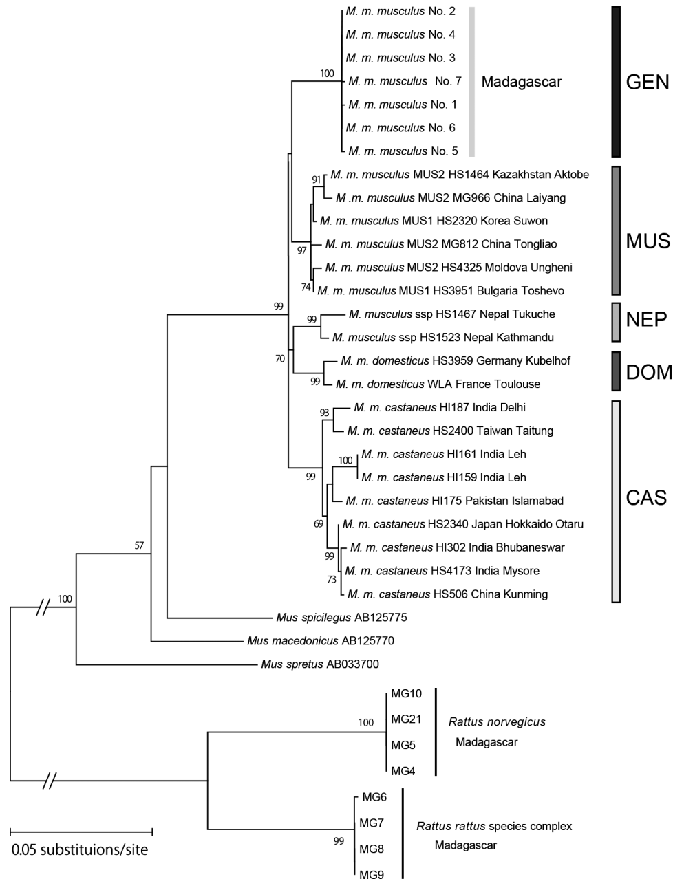
Fig. 5. A ML tree for mitochondrial cytochrome b gene sequences (1,140 bp) of Madagascar mice and those from databases for the four major lineages of M. m. castaneus (CAS), M. m. domesticus (DOM), M. m. musculus (MUS), and Nepal (NEP). Rat species were used as the outgroup taxa. The Madagascar lineage was characterized as M. m. gentilulus (GEN) based on the phylogenetic analyses shown in Figure 3. Bootstrap support values (>50%) are shown at the nodes and were based on 1,000 resampling replicates.
