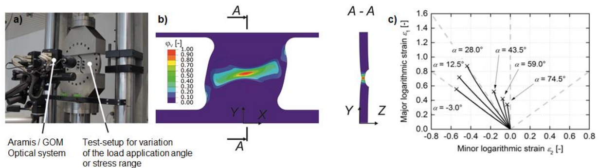
Figure 6. Test setup (a) for testing IFUM- butterfly specimen (b) in a wide range of stress states from tension to shear by variation of the load application angle (c)
