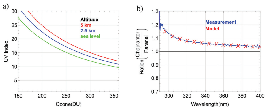
Fig. 6 (a) Change in the UVI with the altitude. The UVI was computed using the UVSPEC model under the conditions observed around noon (SAZ = 5°) at the Paranal Observatory on 09.01.2013 (albedo = 0.1; AOD = 0.15; SSA = 0.7) but assuming different altitudes: 5 km (red line); 2.5 km (blue line); 0 km (green line). (b) Blue line stands for the ratio between spectra estimated at SAZ = 5° from our ground-based measurements on the Chajnantor Plateau (on 15.01.2013) and at the Paranal Observatory (on 09.01.2013). Red crosses stand for the ratio between spectra computed by using the UVSPEC model at SAZ = 5° and at different altitudes (5100 m and 2635 m).
