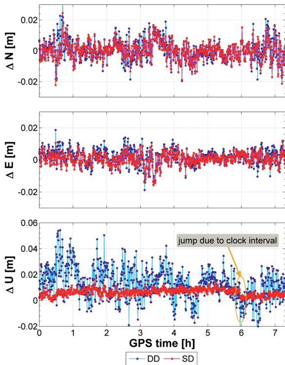
Figure 5: Comparison of kinematic coordinates for the 290 m baseline between Kopfermann and Meitner building for the North (top), East (middle), and Up (down) component in [m]. Blue: computed with standard DD, red computed with common clock single-differences.
