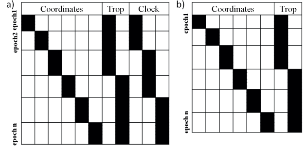
Figure 3: Non zero-elements in the design matrices (black), Case of between-station single differences (a), same situation for DD (b).
