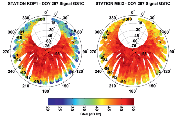
Figure 2: Skyplots with color-coded carrier to noise density ratios, for the Kopfermann (left) and Meitner building (right), respectively. A common color scale is applied. Blue colors indicate weak signals.
