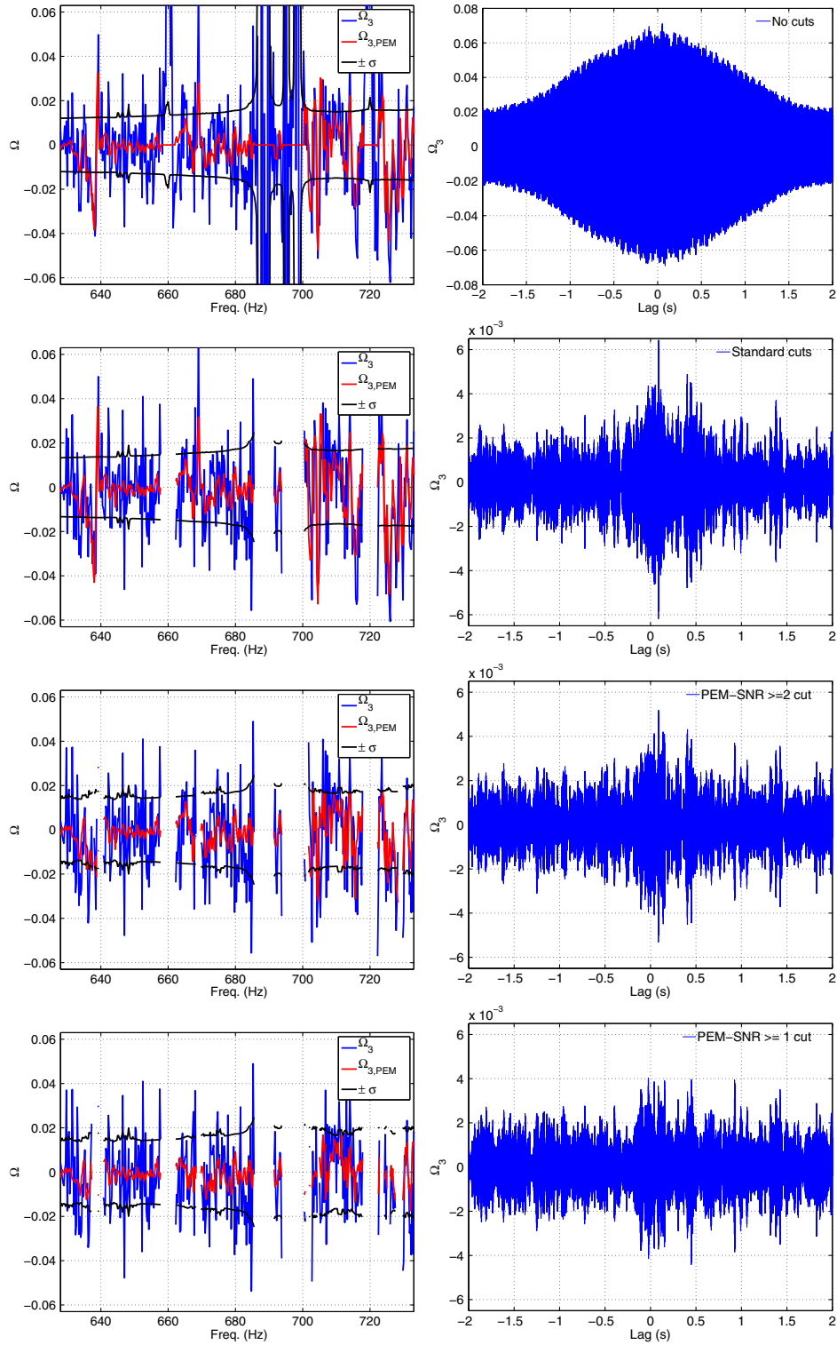
FIG. 5 (color online). Plots of \hat{\Omega}_3(f) and \hat{\Omega}_{3,\text{PEM}}(f) (left panels), and the inverse Fourier transform of \hat{\Omega}_3(f) (right panels), for the (noisiest) 628–733 Hz subband after various stages of noise removal were applied to the data. The four rows correspond to the four different stages of cleaning defined in Table I. (The top right plot has y-axis limits 13 \times greater than the other three.)
