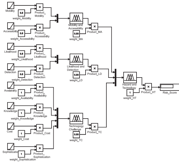
Fig. 14. MATLAB-Simulink model for the estimation of the risk from the inputs ML, TC, and LoD.
