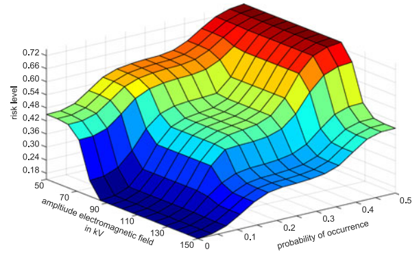
Fig. 15. Risk level in dependence on the field and probability of occurrence of an IEMI source by Peikert [9].
