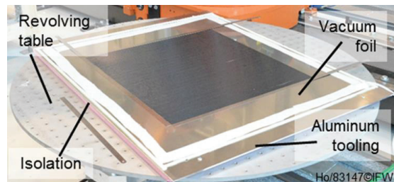
Fig. 3. Experimental set-up.
