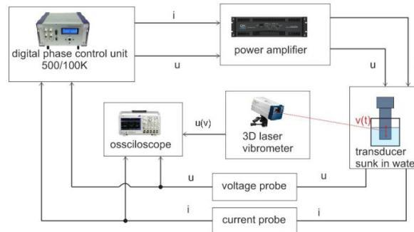
Figure 5. Experimental setup for observation of ultrasonic-induced cavitation.
